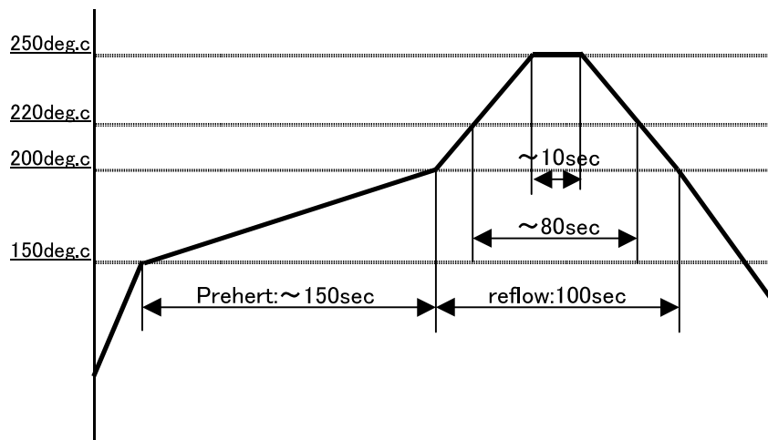
Reflow profile #1
