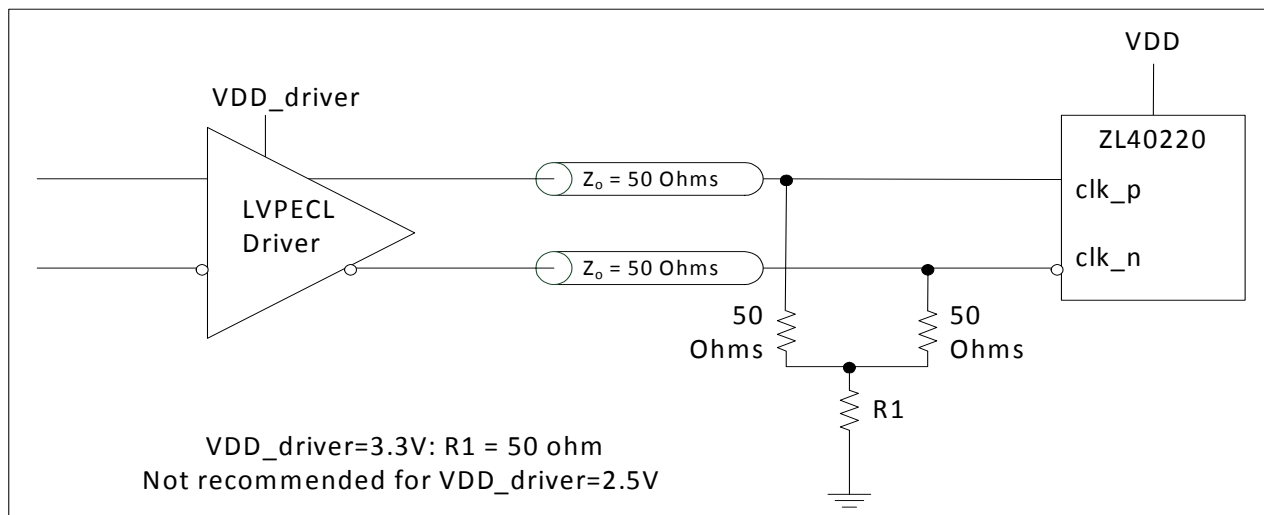
Figure 4 - LVPECL Input DC Coupled Thevenin Equivalent
