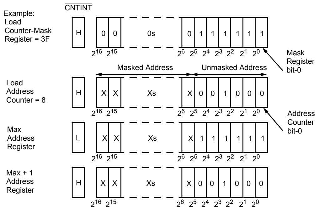
Figure 2. Programmable Counter-Mask Register Operation [1, 20]
