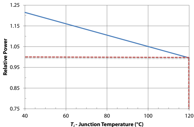
Relative Power vs Junction Temperature ( T_j ) I_f = 18\text{ A} , normalized to 120^\circ\text{C}
