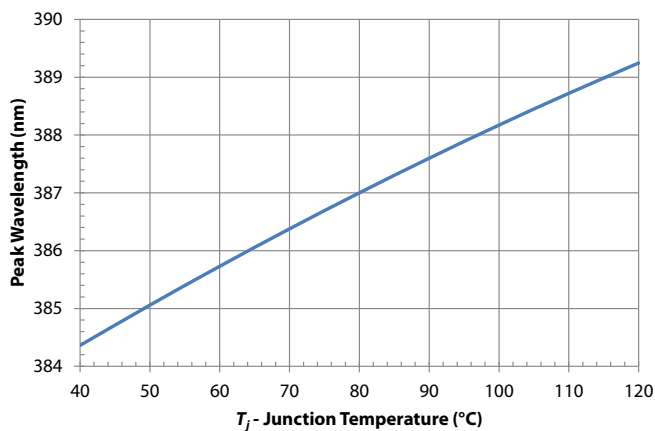
Peak Wavelength vs Junction Temperature ( T_j )
