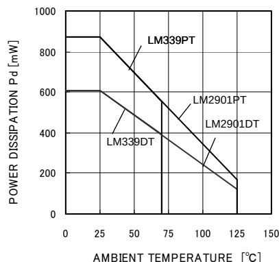
LM339DT/PT LM2901DT/P
