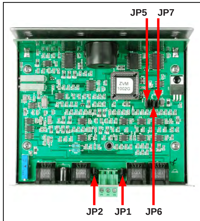
Figure 5. Jumper locations
