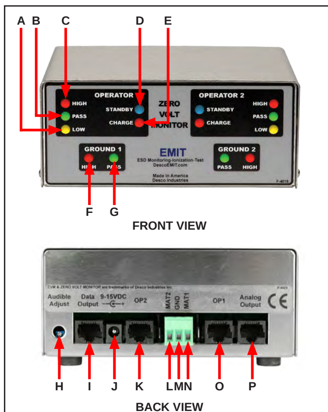
Figure 2. Zero Volt Monitor features and components
