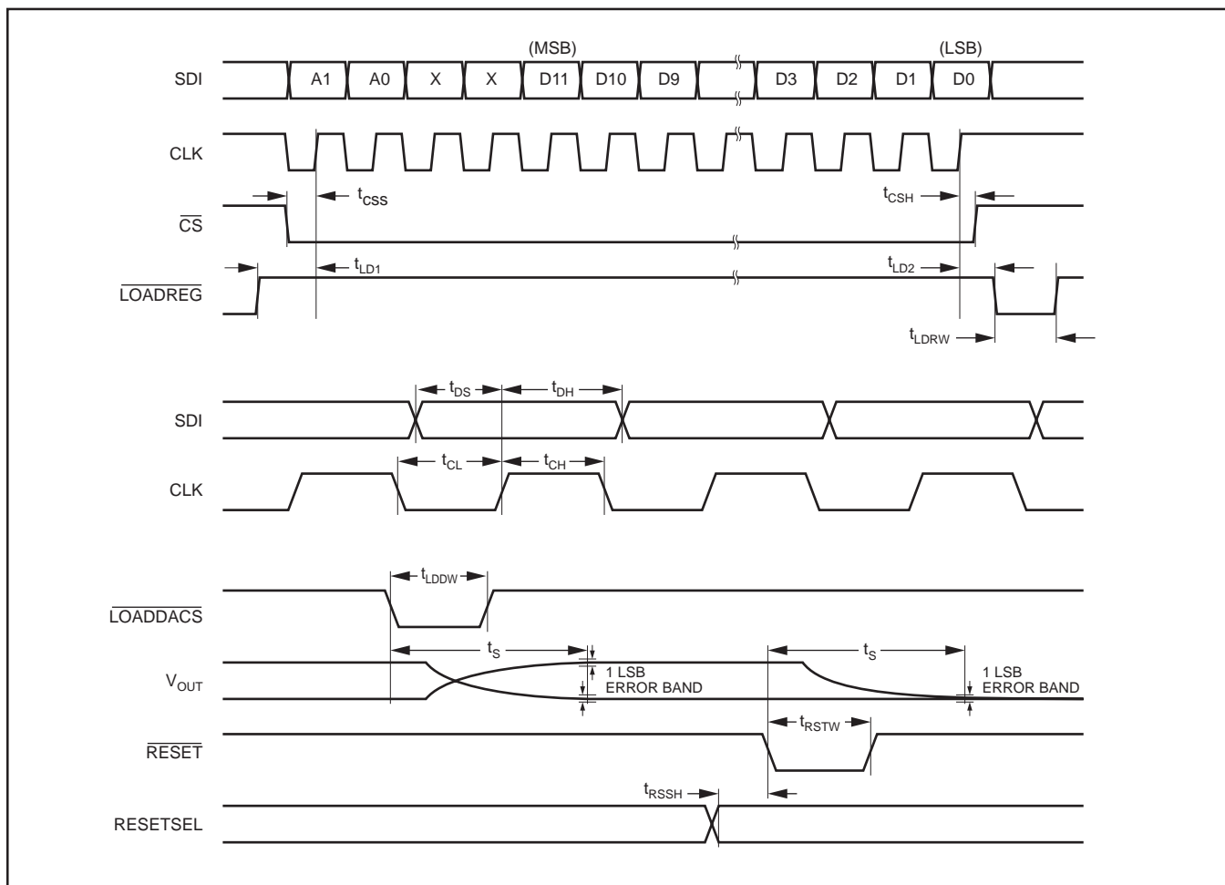
FIGURE 3. DAC7615 Timing.
