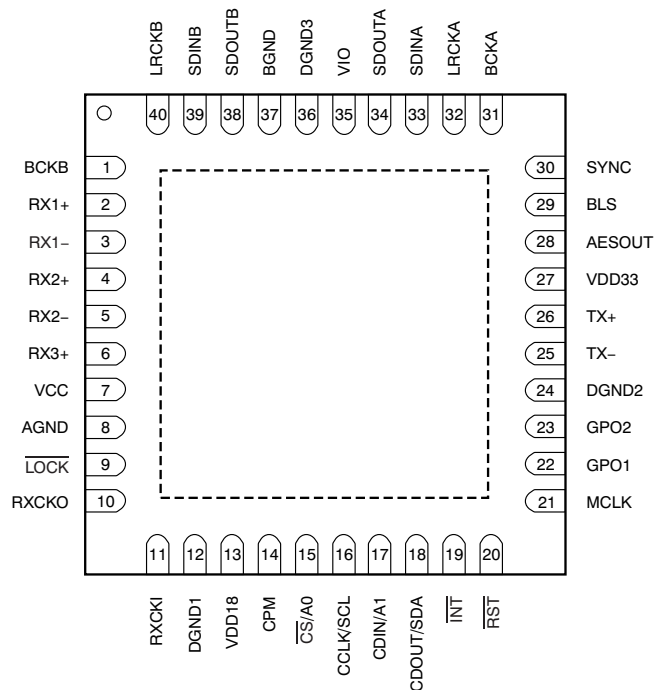
RKP PACKAGE QFN-40 (Top View)
