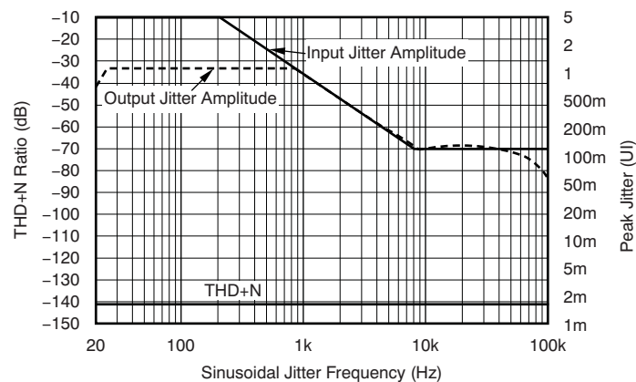
Figure 70. DIR Jitter Tolerance Plot
