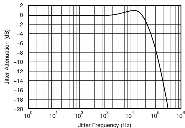
Figure 69. DIR Jitter Attenuation Characteristics
