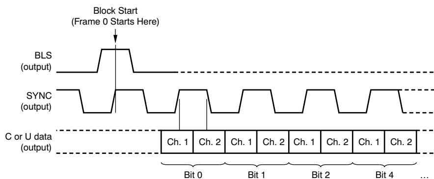
Figure 71. DIR Channel Status and User Data Serial Output Format Via the GPO Pins
