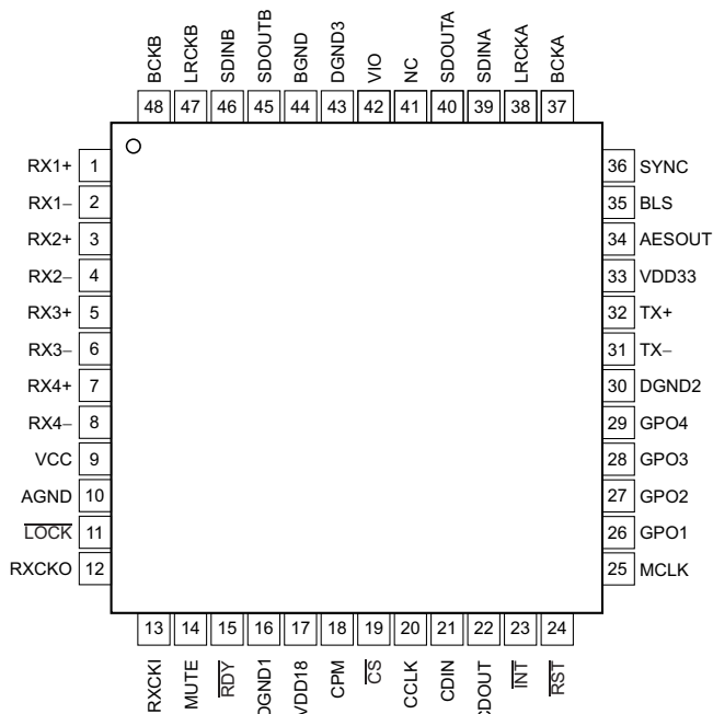
PFB PACKAGE TQFP-48 (Top View)
