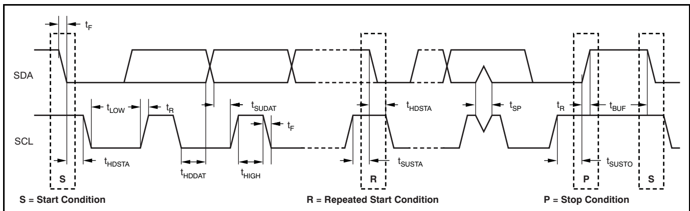
Figure 3. I²C Standard and Fast Mode Timing
