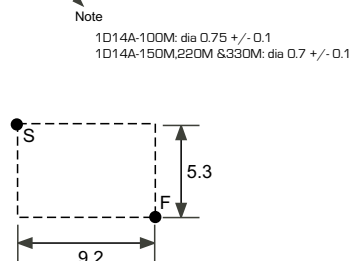
Footprint
