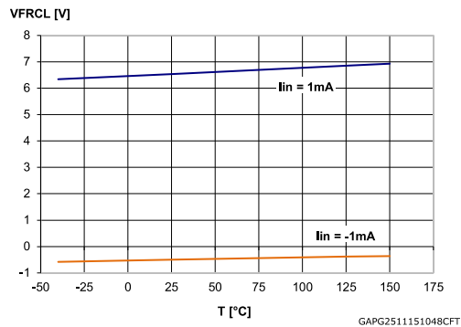
Figure 21: FaultRST Input clamp voltage
