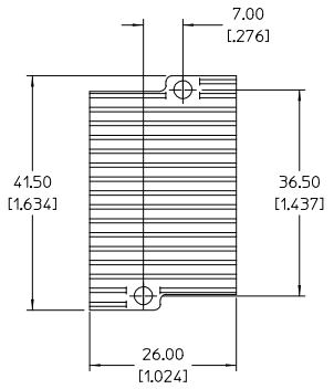
X-FLOW (XF) (HEAT SINK ONLY SHOWN)
