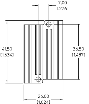
LONGITUDINAL FLOW (LF) (HEAT SINK ONLY SHOWN)
