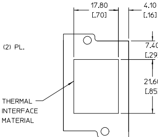
BOTTOM VIEW (HEATSINK AND THERMAL INTERFACE MATERIAL ONLY)
