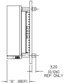
J-LEAD MOUNT
