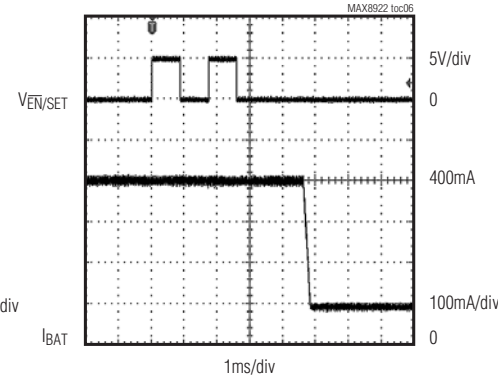
CHARGE CURRENT WITH TWO EN/SET PULSES
