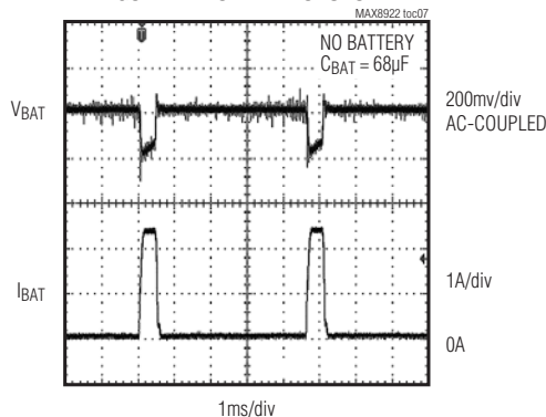
GSM TRANSIENT RESPONSE
