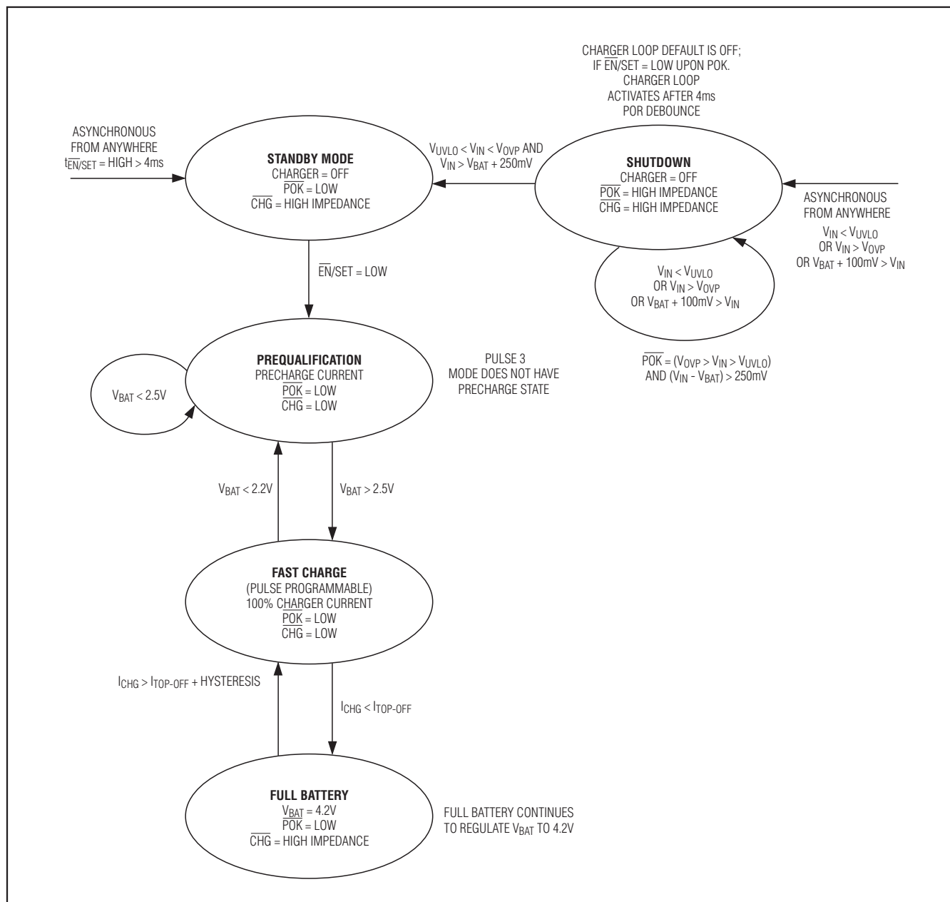
Figure 2. Charger State Diagram
