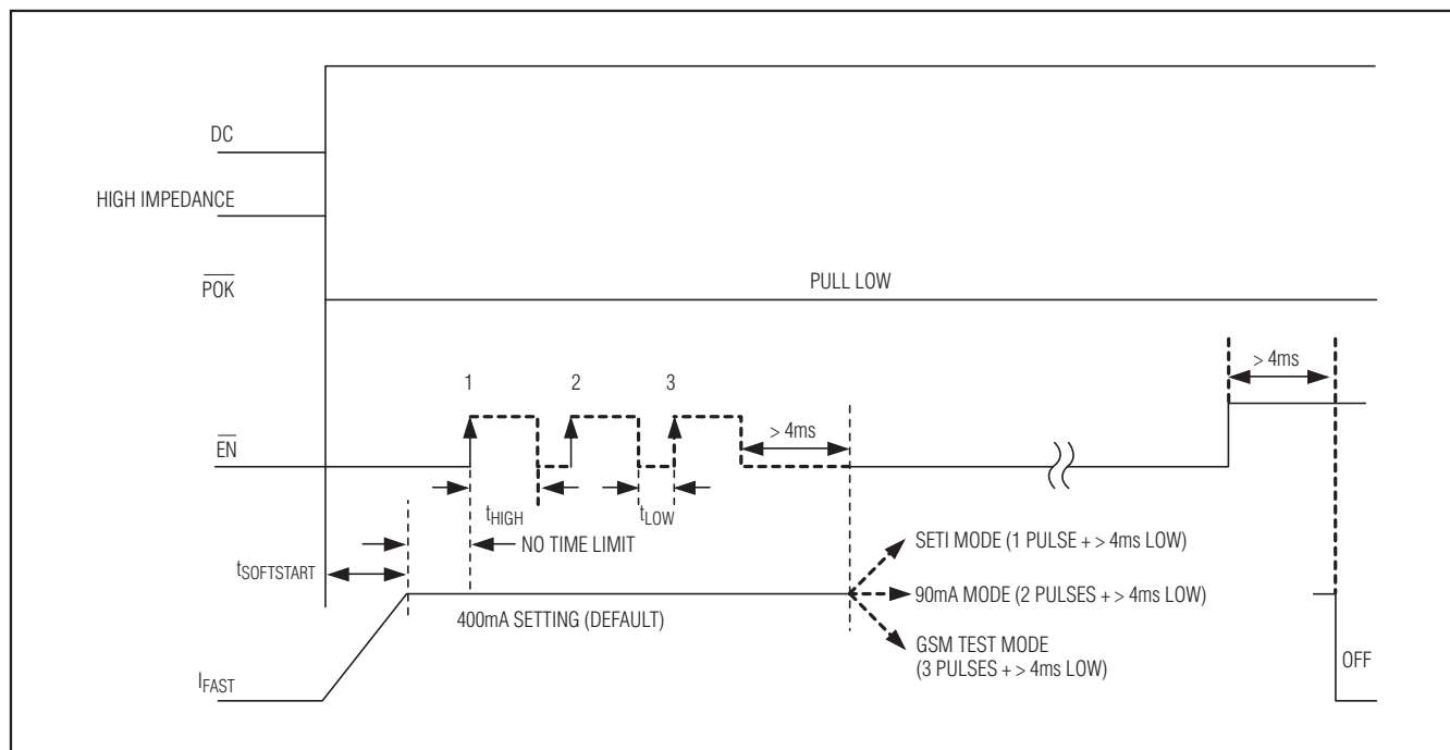
Figure 3. Charge-Current Programming
