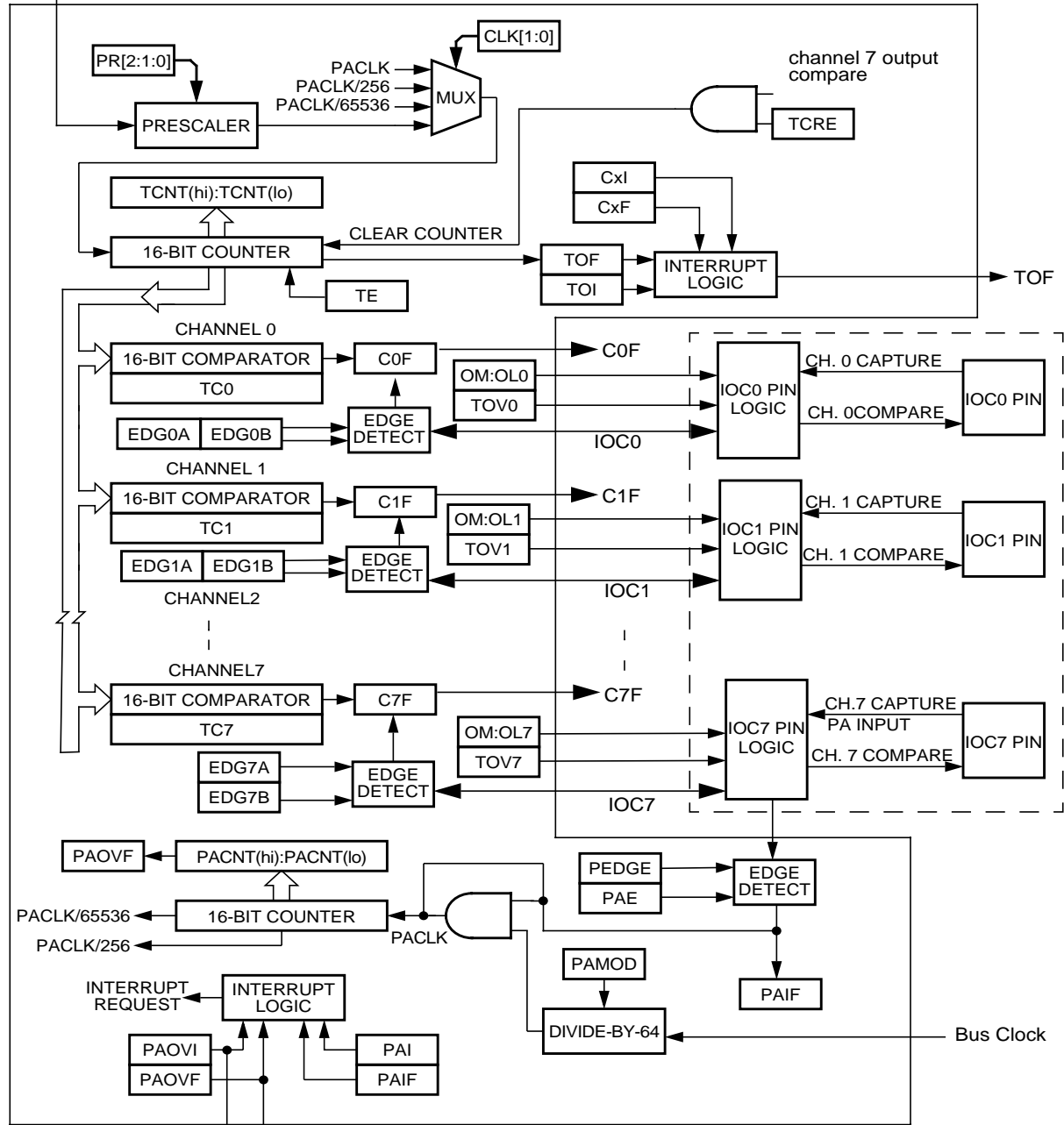
Figure 14-30. Detailed Timer Block Diagram
