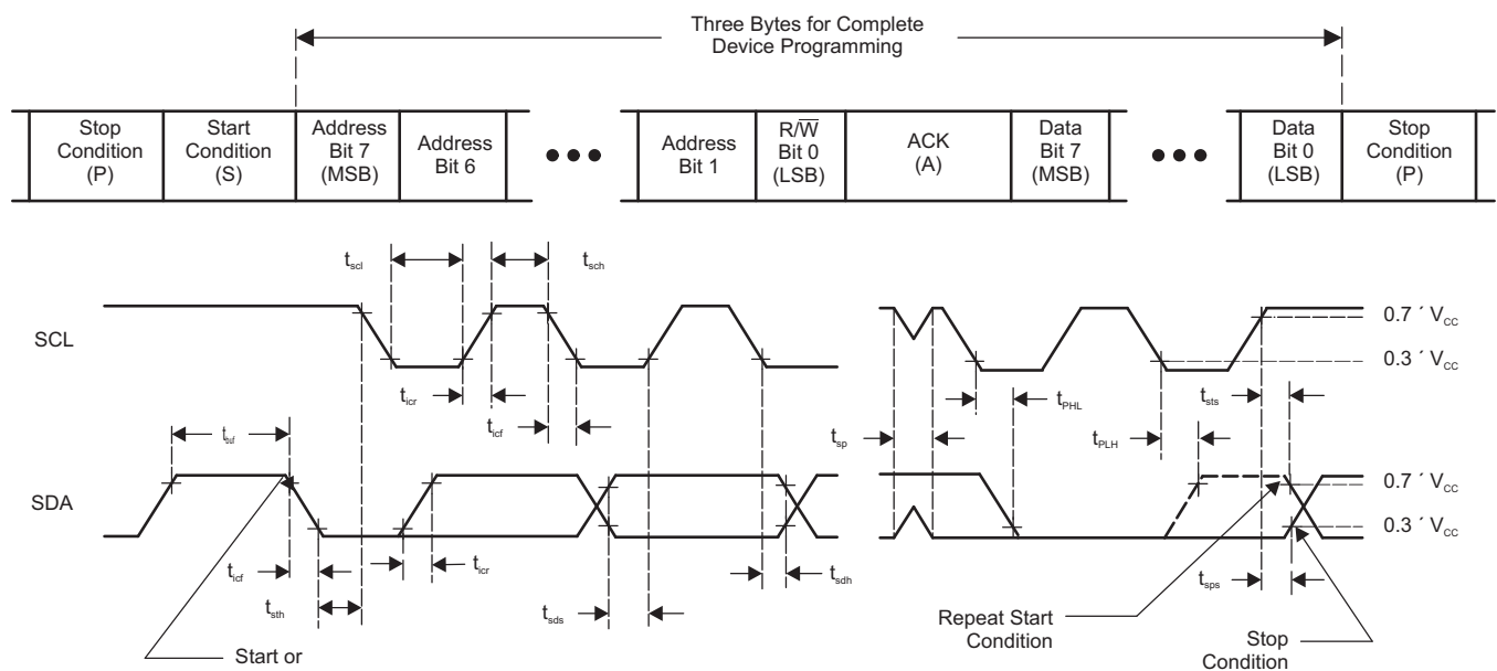
VOLTAGE WAVEFORMS
