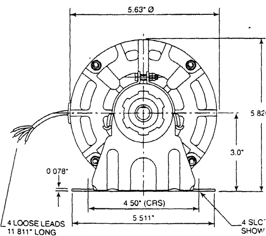
FRAME B48 MOTOR, RESILIENT BASE MOUNTING, O BS 2048
