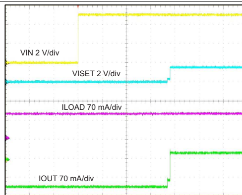
Figure 12. Battery Removal
