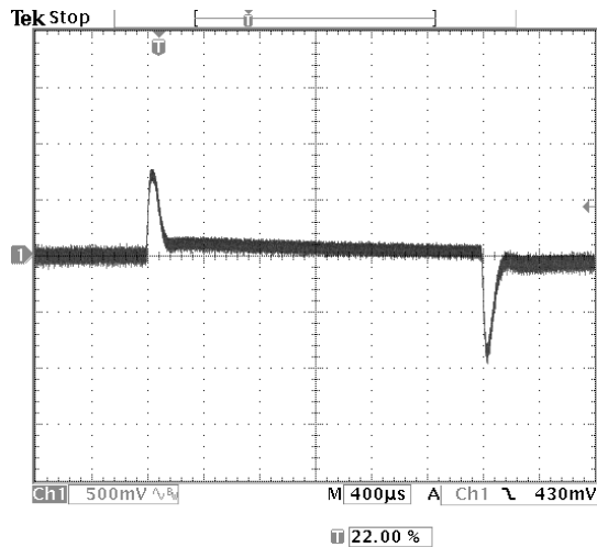
Photo 7: Transient Response 50% to 100% Vin=24V, Iout = 2.9 to 5.8A Cout=1uF Ceramic + 10uF Tantalum
