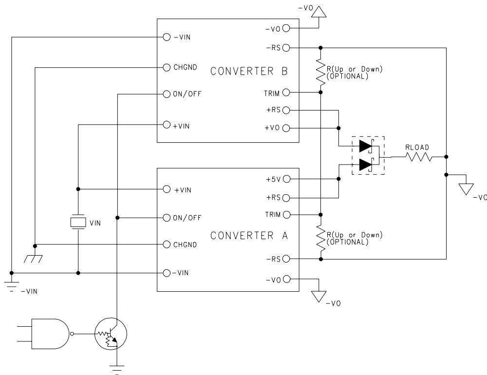
Figure 6: Paralleling Converters
