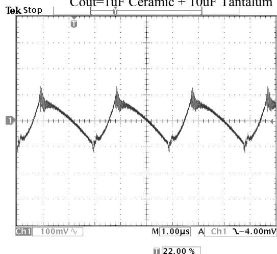
Photo 11: Output Voltage Ripple (Spike) Vin=24V, Iout = 5.8A Cout=1uF Ceramic + 10uF Tantalum
