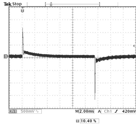
Photo 8: Transient Response 10% to 100% Vin=24V, Iout = 0.6 to 5.8A Cout=1uF Ceramic + 10uF Tantalum
