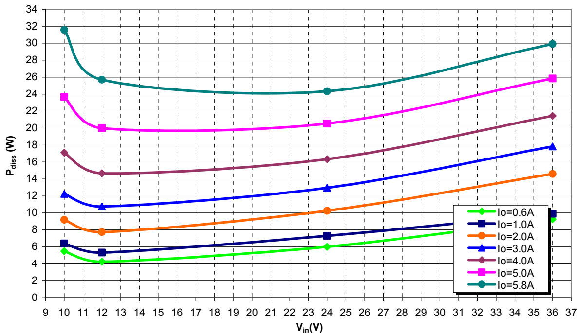
Graph 3: LV12S26-150 Power Dissipation vs. Input Voltage
