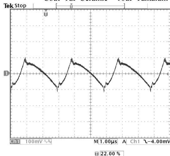
Photo 10: Output Voltage Ripple (20 MHz BW) Vin=24V, Iout=5.8A Cout=1uF Ceramic + 10uF Tantalum
