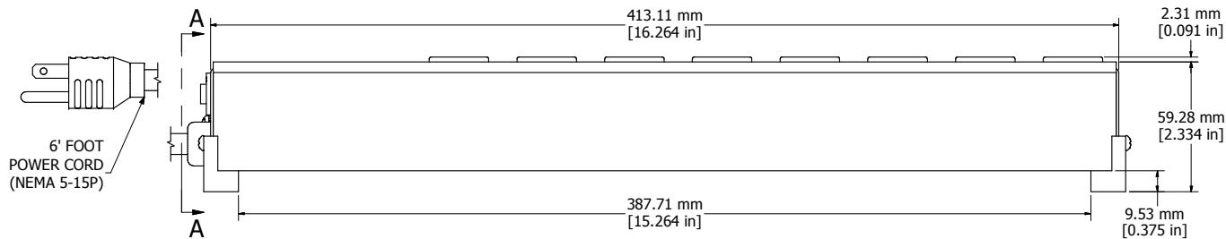
ASSEMBLY - VIEW FROM SIDE
