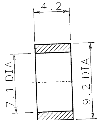
Retaining Ring
