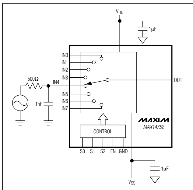
Figure 12. Input Slew-Rate Limit
