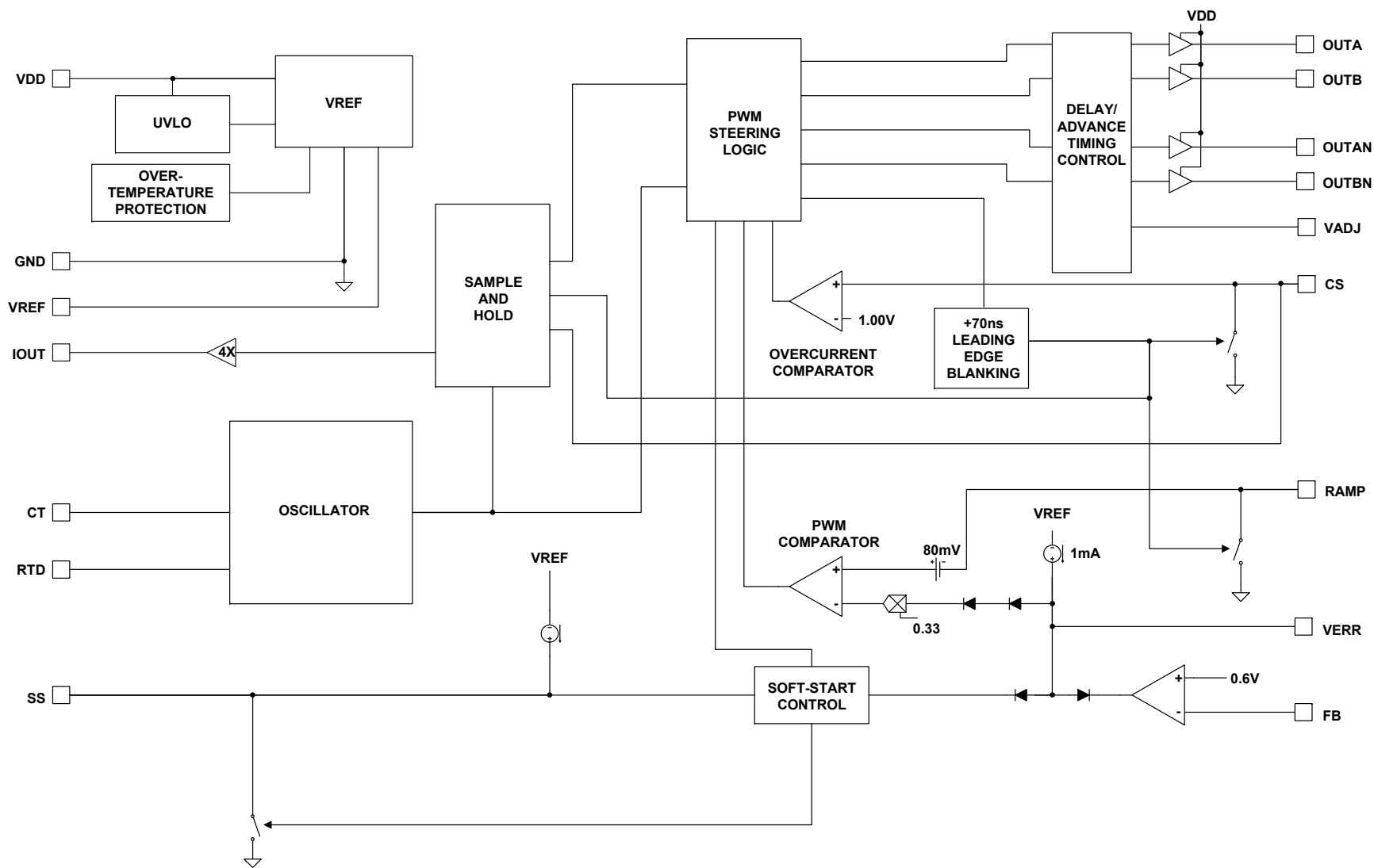
FIGURE 1. FUNCTIONAL BLOCK DIAGRAM
