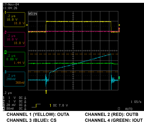
FIGURE 8. CS INPUT vs IOU
