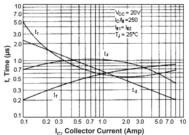
Switching Time
