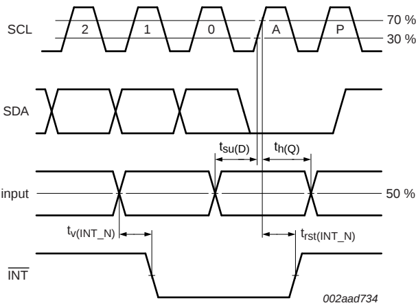
Fig 25. Expanded view of read input port register
