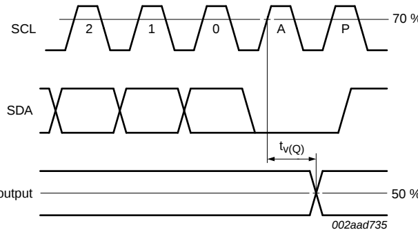
Fig 26. Expanded view of write to output port register
