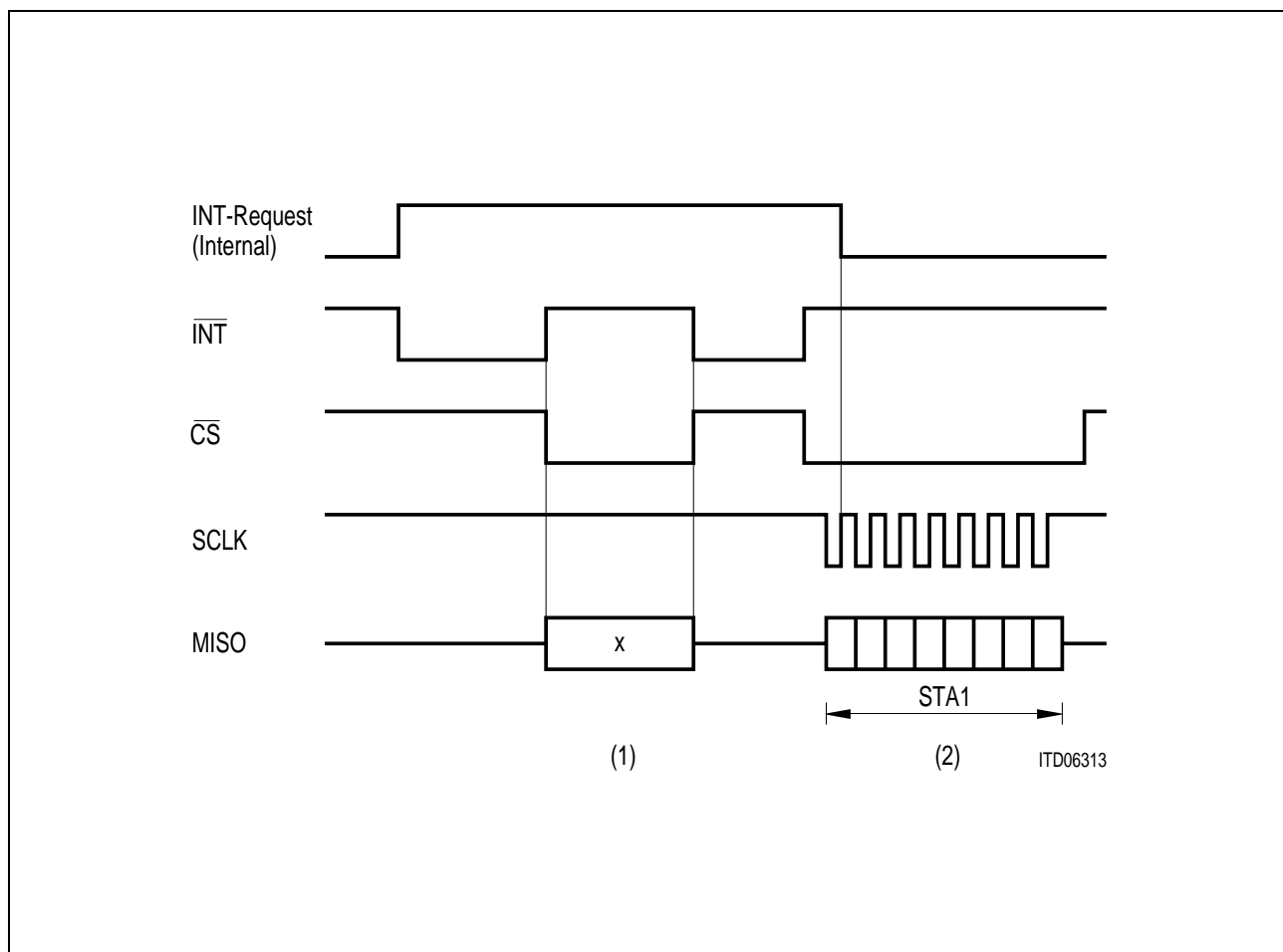
Figure 18 Interrupt Output
