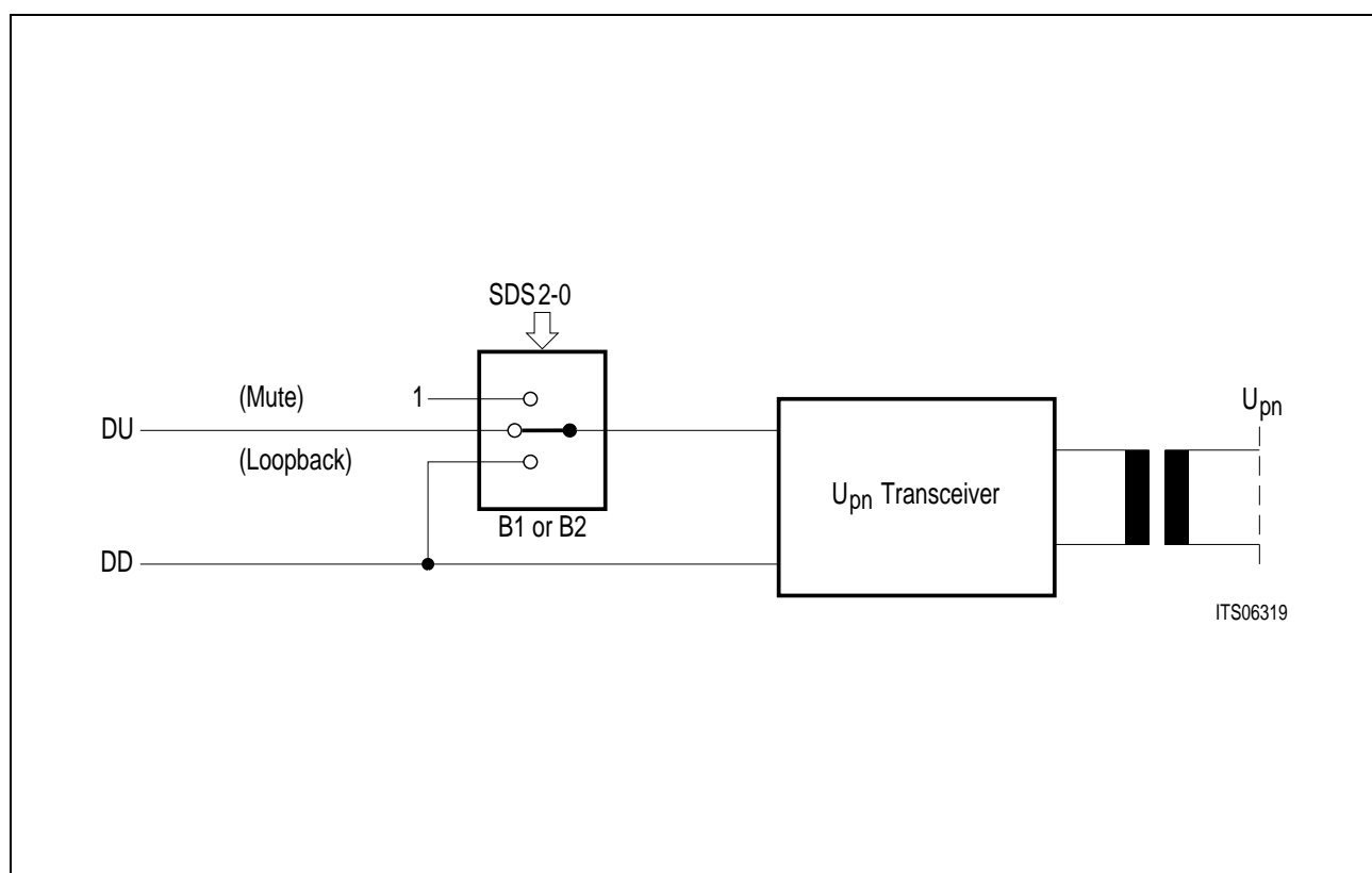
Figure 23 B-Channel Manipulation
