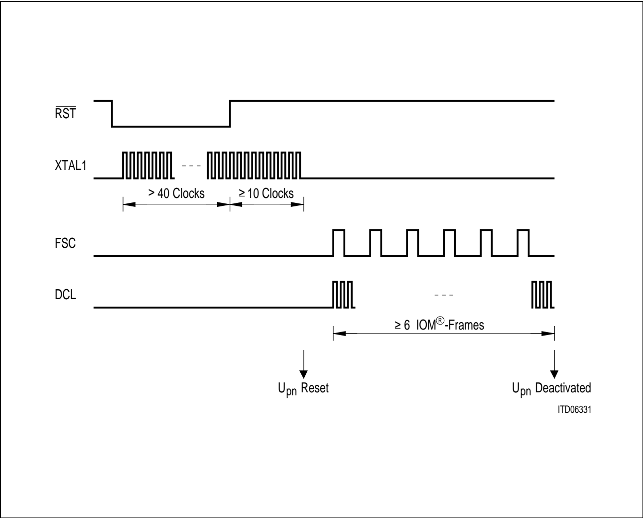
Figure 41 Reset
