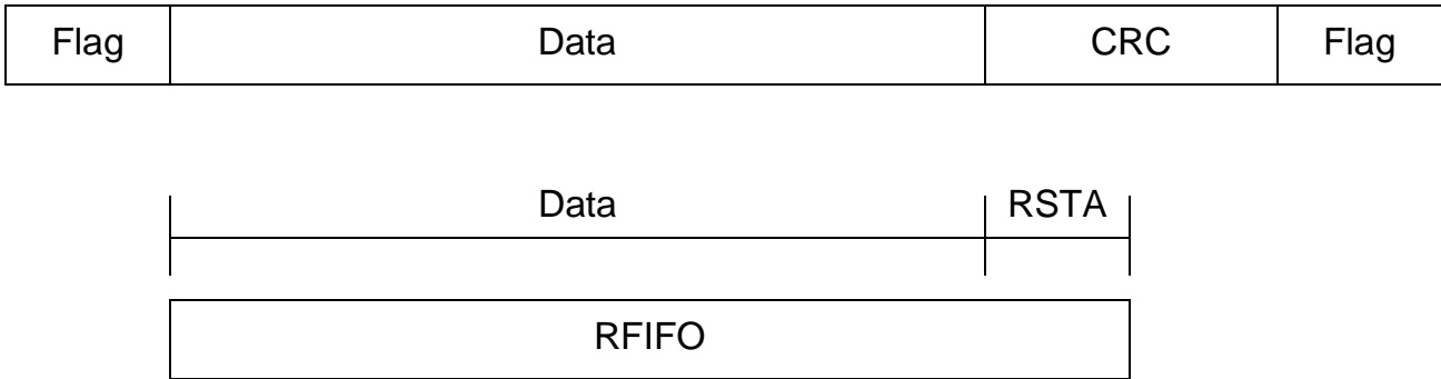
Figure 29 HDLC-Receiver Format
