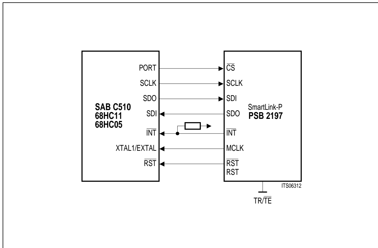
Figure 17 Interfacing the SmartLink-P to a Siemens SAB C510x or Motorola Microprocessor
