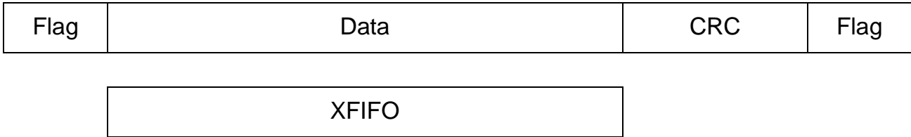
Figure 28 HDLC-Transmitter Format
