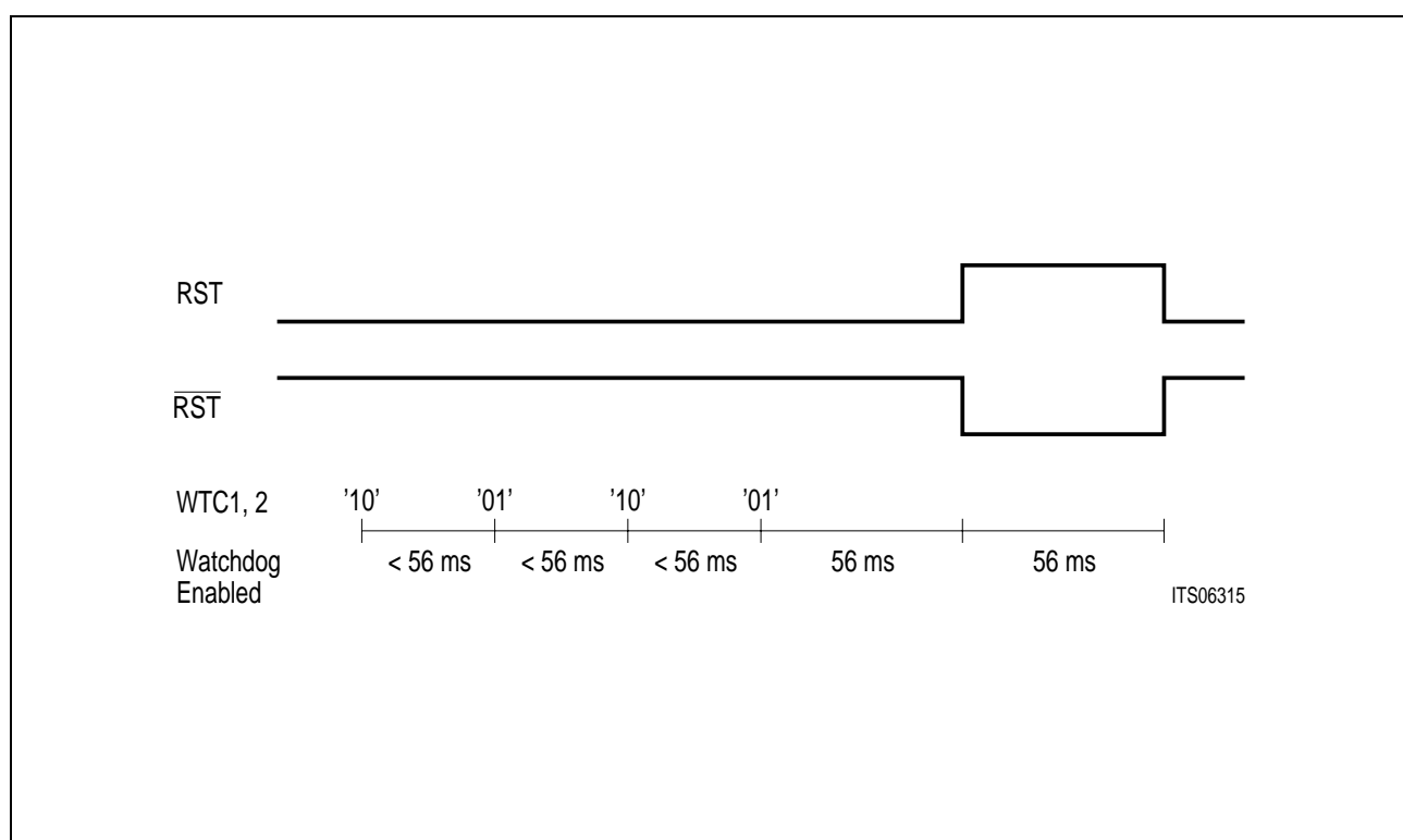
Figure 20 Watchdog Operation
