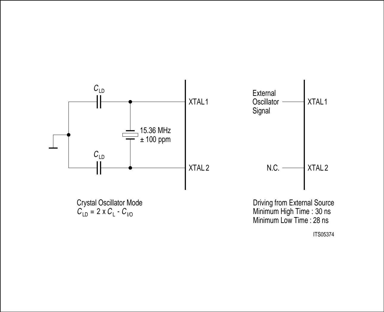
Figure 54 Oscillator Circuits
