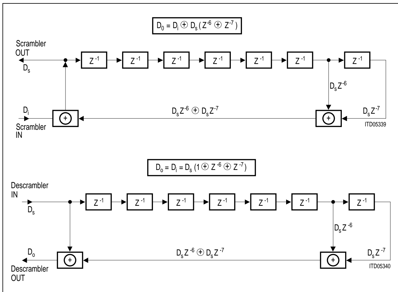
Figure 25 Scrambler/Descrambler
