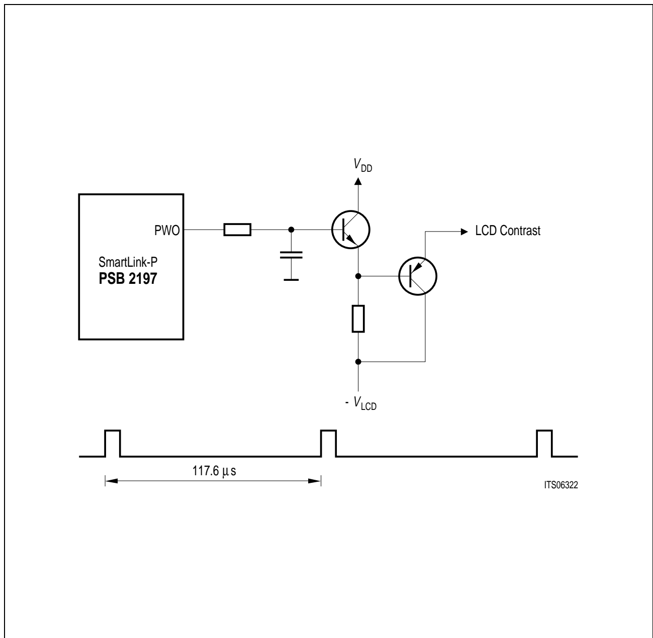
Figure 30 LCD-Contrast Control
