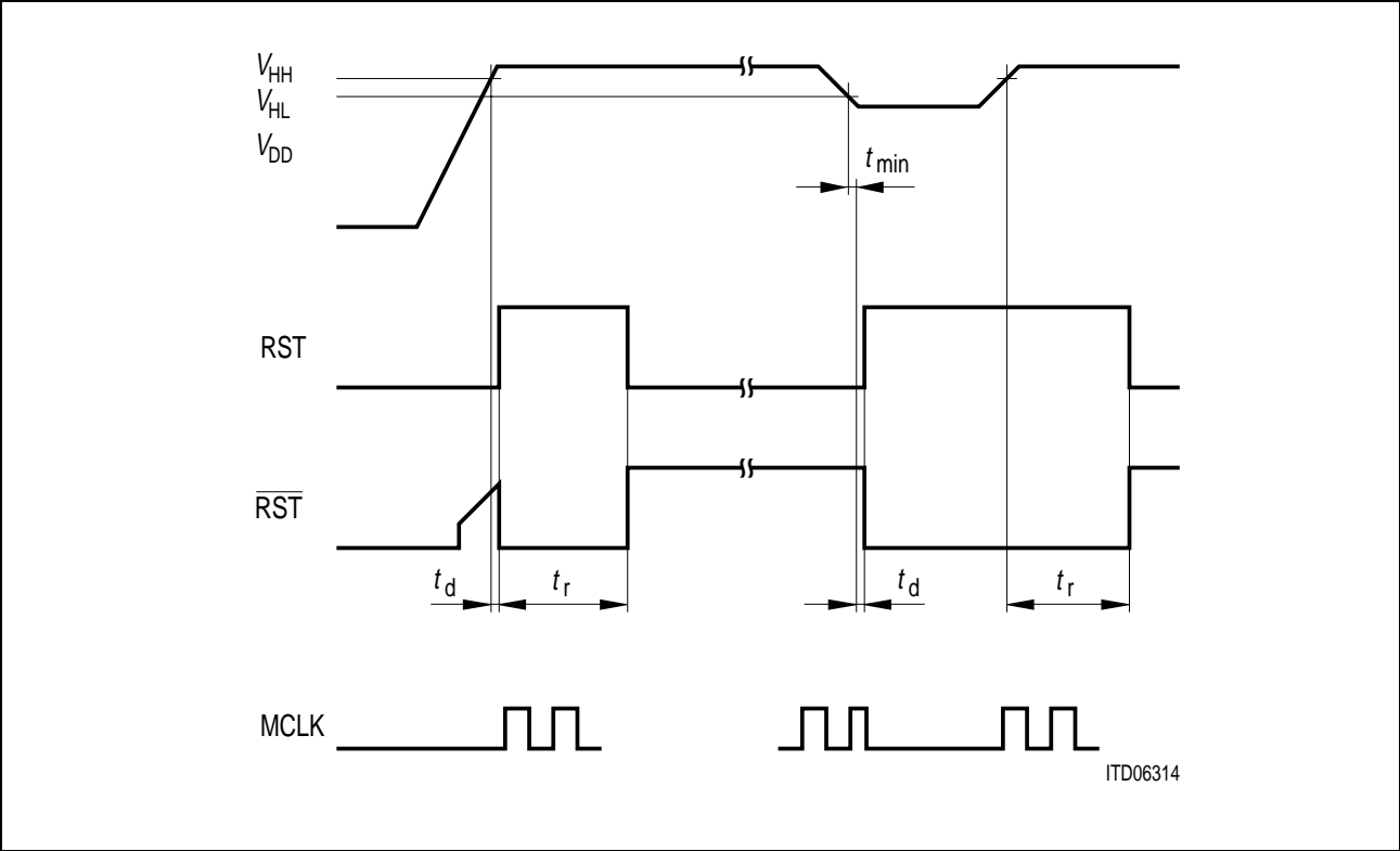
Figure 59 Undervoltage Detection
