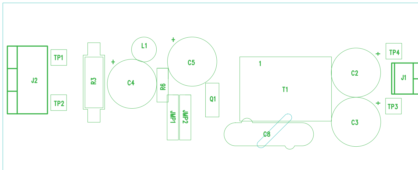
Figure 14. Top Assembly Drawing
