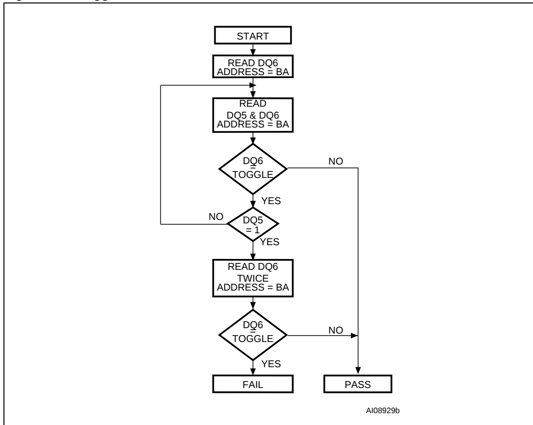
Figure 7. Toggle flowchart
