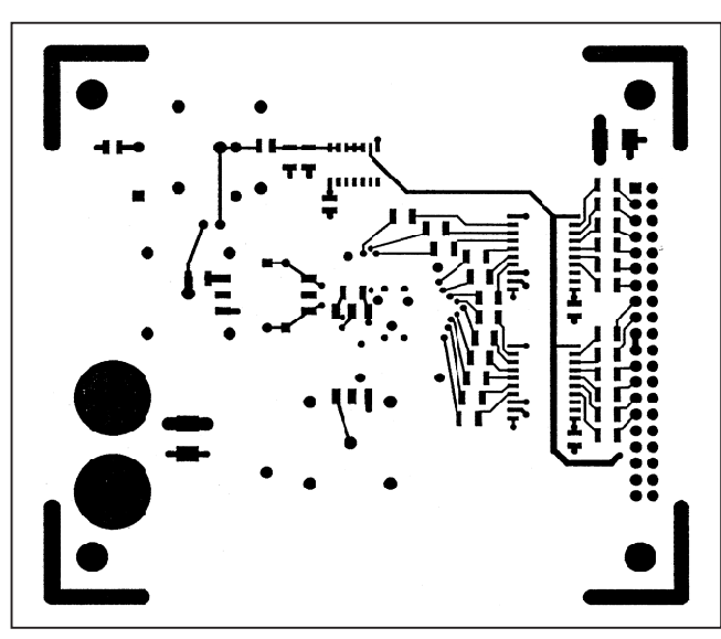
Figure 22. AD6640ST/PCB Bottom Side Copper (Positive)
