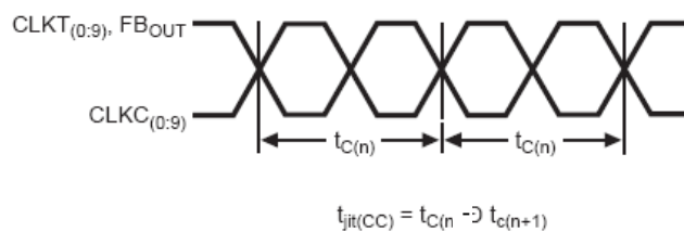
Figure 2. Cycle-to-cycle Jitter
