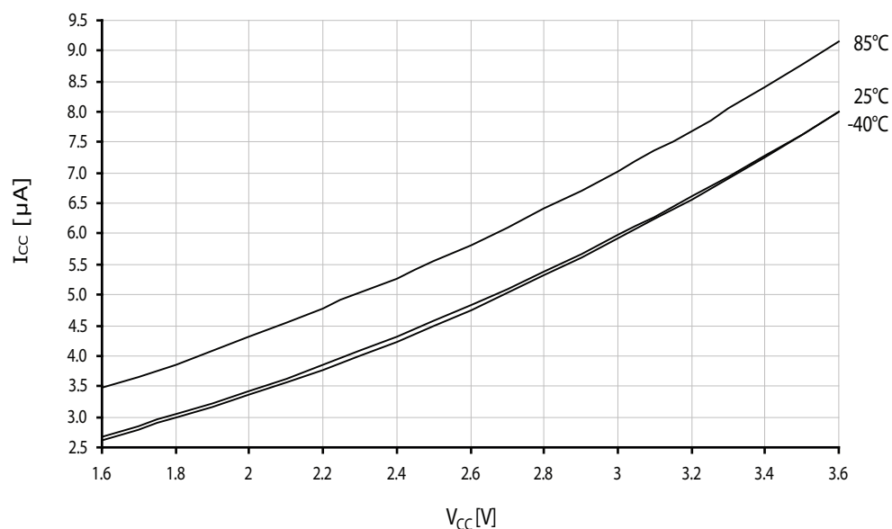
Figure 37-190. Standby supply current vs. V_{CC} .
