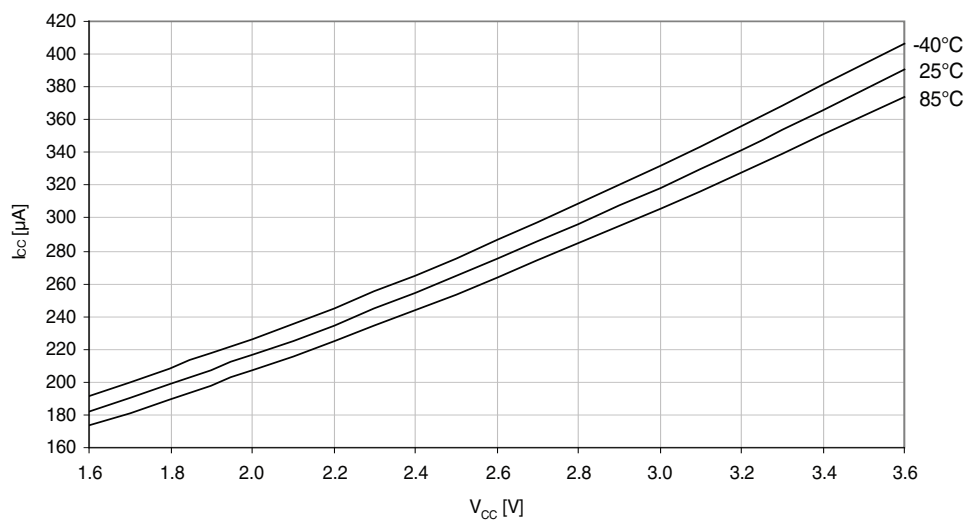
Figure 37-97. Idle mode supply current vs. V_{CC} .
