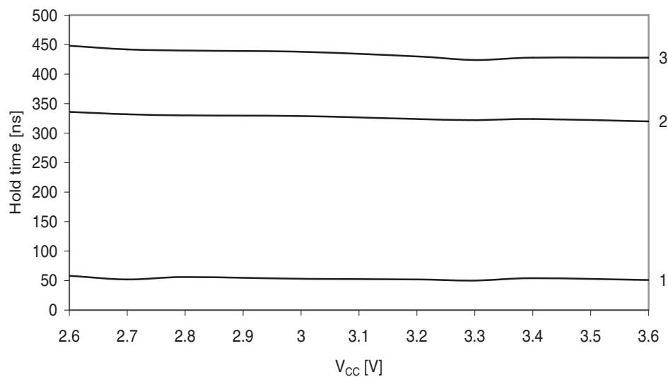
Figure 37-169. SDA hold time vs. supply voltage.
