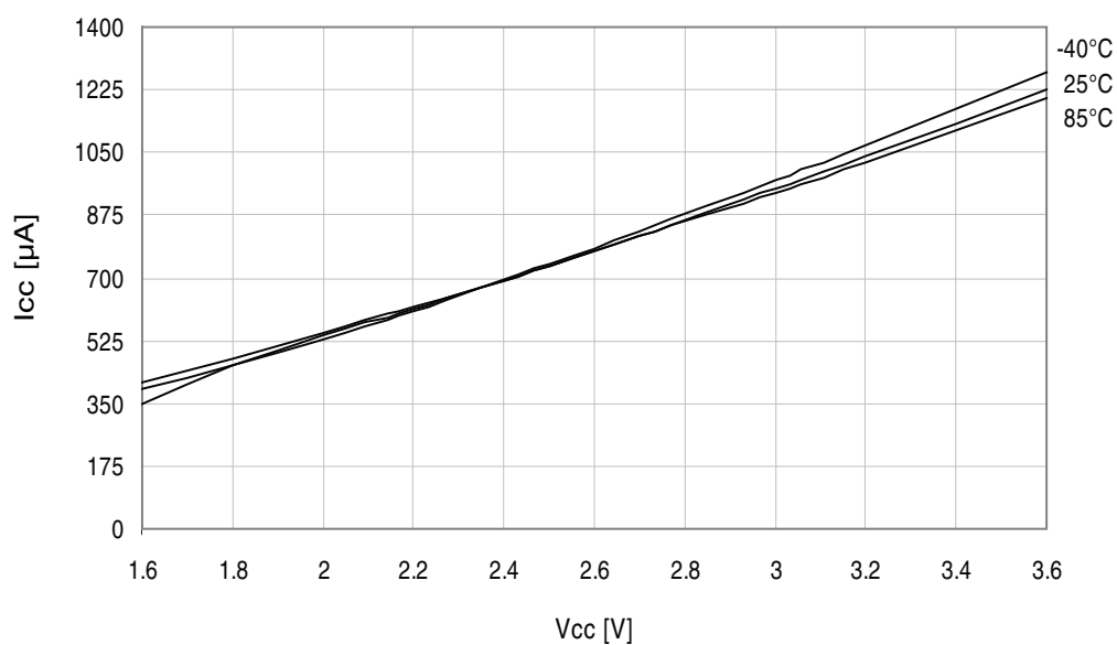
Figure 37-261. Active mode supply current vs. V_{CC} .
