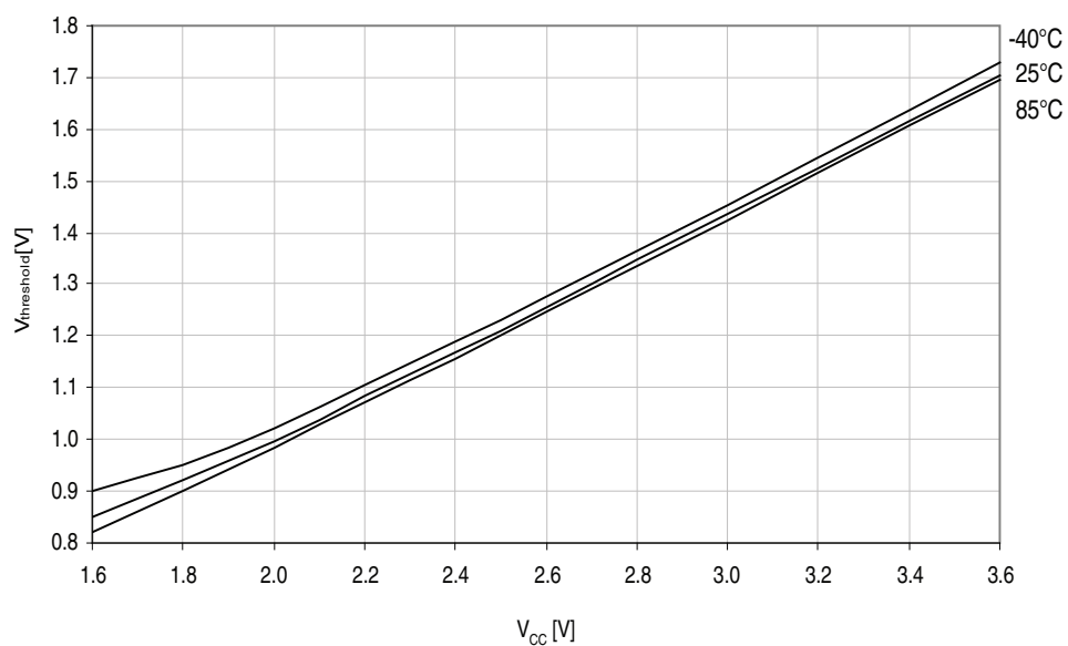
Figure 37-33. I/O pin input threshold voltage vs. V_{CC} . V_{IH} I/O pin read as "1".
