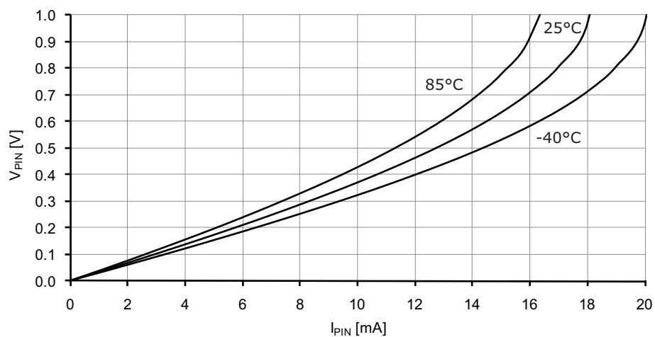
Figure 37-113. I/O pin output voltage vs. sink current.
