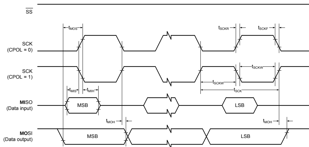
Figure 36-12. SPI timing requirements in master mode.
