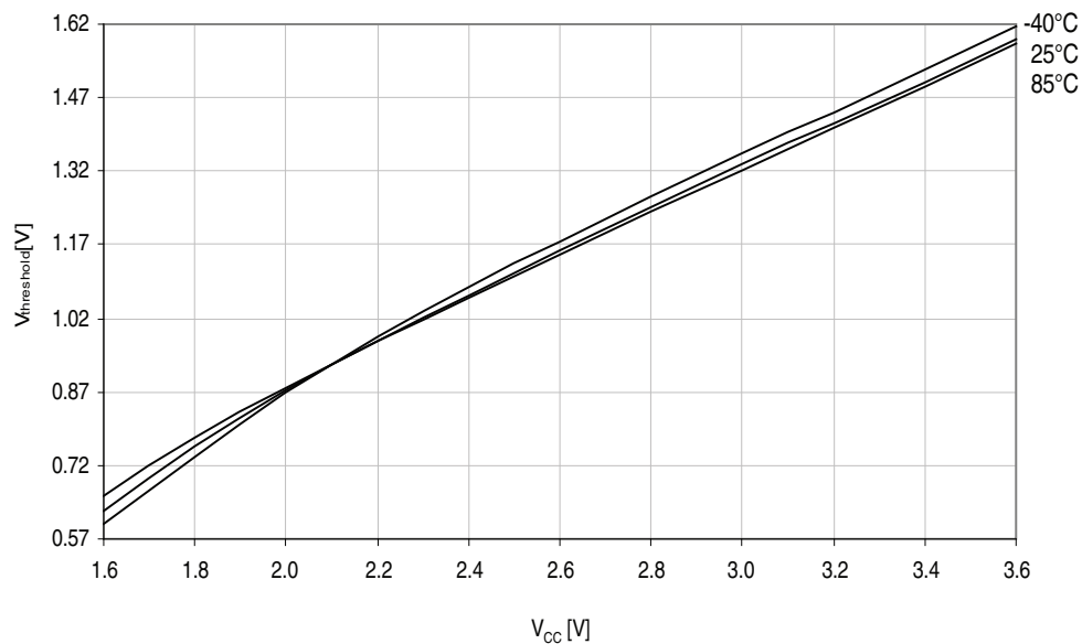
Figure 37-34. I/O pin input threshold voltage vs. V_{CC} . V_{IL} I/O pin read as "0".
