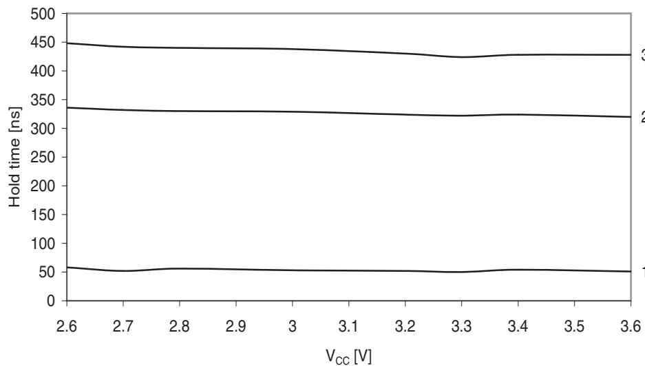
Figure 37-84. SDA hold time vs. supply voltage.
