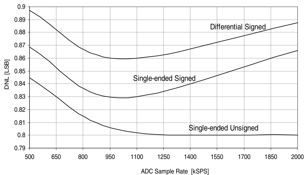
Figure 37-40. DNL error vs. sample rate. T = 25\text{ }^{\circ}\text{C} , V_{CC} = 3.6\text{V} , V_{REF} = 3.0\text{V} external.
