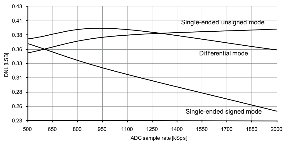
Figure 37-210. DNL error vs. sample rate. T = 25\text{ }^{\circ}\text{C} , V_{CC} = 2.7\text{V} , V_{REF} = 1.0\text{V} external.
