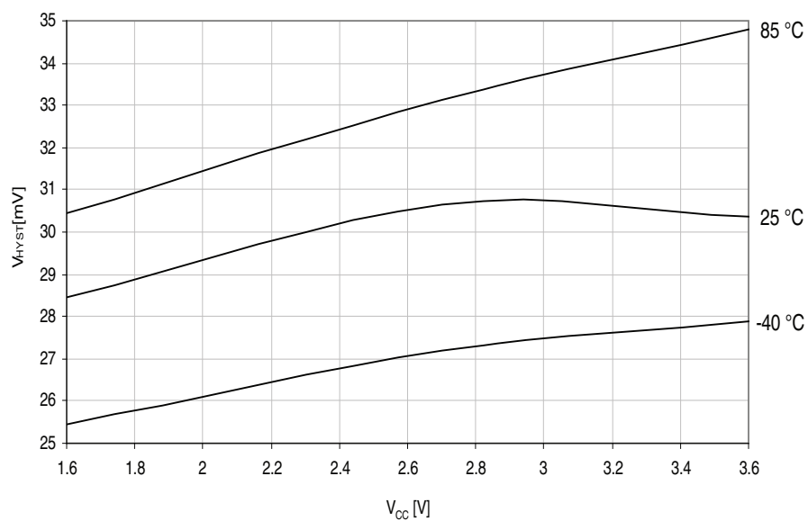
Figure 37-54. Analog comparator hysteresis vs. V_{CC} . High-speed mode, large hysteresis.
