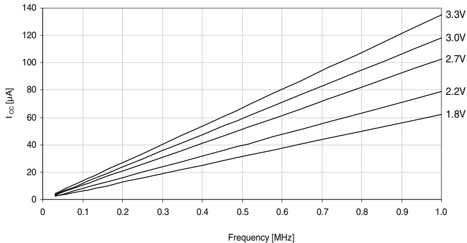
Figure 37-8. Idle mode supply current vs. frequency. f_{SYS} = 0 - 1\text{MHz} external clock, T = 25^\circ\text{C} .
