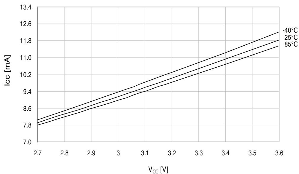
Figure 37-262. Active mode supply current vs. V_{CC} .
