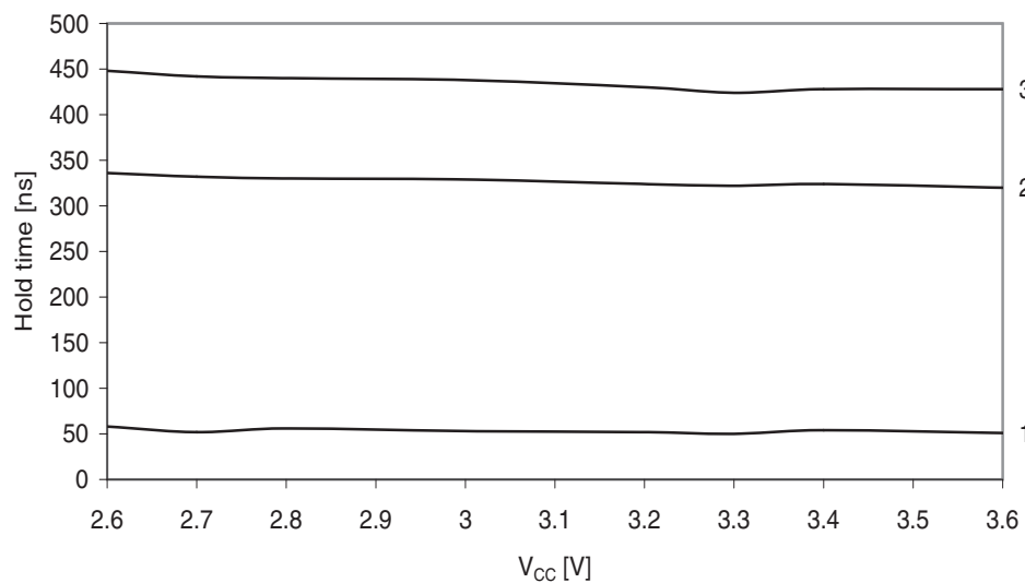
Figure 37-337. SDA hold time vs. supply voltage.
