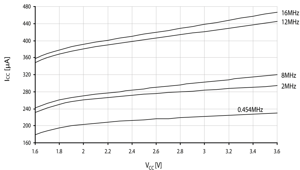
Figure 37-190. Standby supply current vs. V_{CC} .
