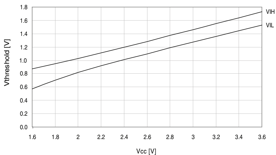
Figure 37-202. I/O pin input threshold voltage vs. V_{CC} .
