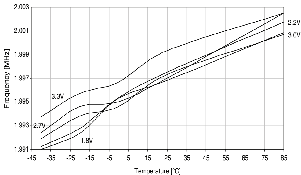
Figure 37-74. 2MHz internal oscillator frequency vs. temperature.
