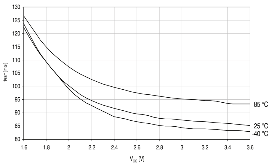
Figure 37-62. Minimum Reset pin pulse width vs. V_{CC} .
