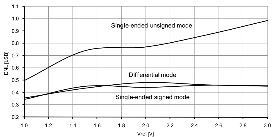
Figure 37-209. DNL error vs. external V_{REF} . T = 25\text{ }^{\circ}\text{C} , V_{CC} = 3.6\text{V} , external reference.
