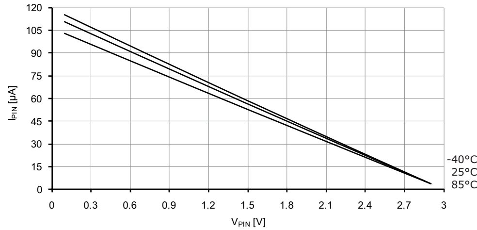
Figure 37-192. I/O pin pull-up resistor current vs. input voltage. V_{CC} = 3.0V .
