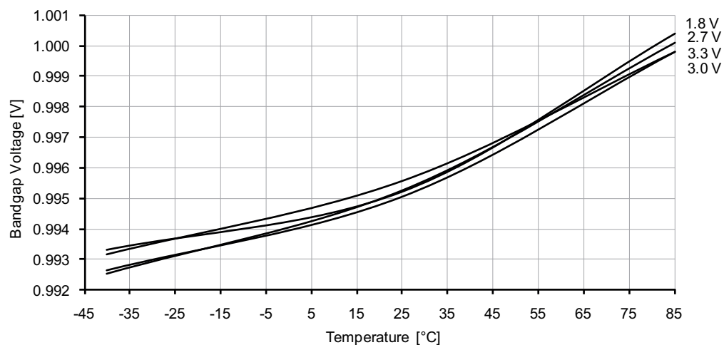
Figure 37-229. ADC/DAC Internal 1.0V reference vs. temperature.
