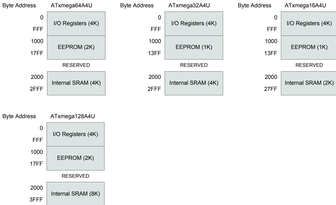
Figure 7-3. Data memory map (Hexadecimal address).
