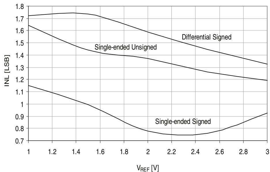
Figure 37-121. INL error vs. external V_{REF} .
