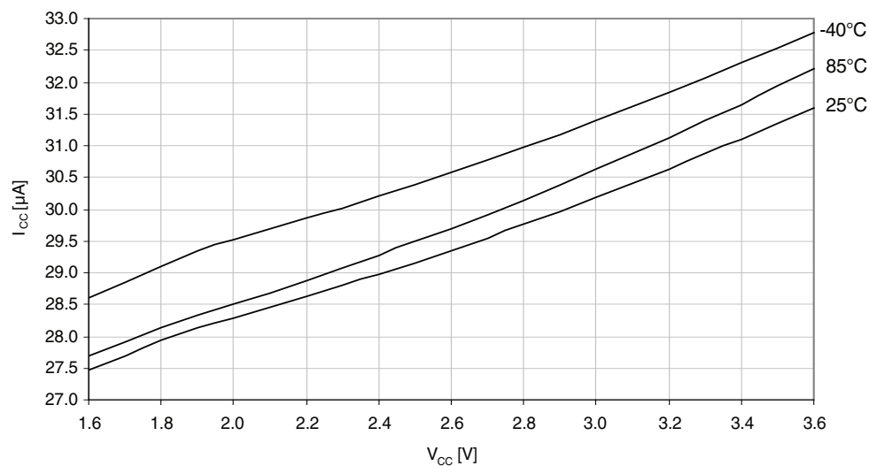
Figure 37-10. Idle mode supply current vs. V_{\text{CC}} .
