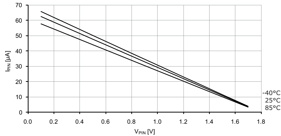
Figure 37-191. I/O pin pull-up resistor current vs. input voltage. V_{CC} = 1.8V .
