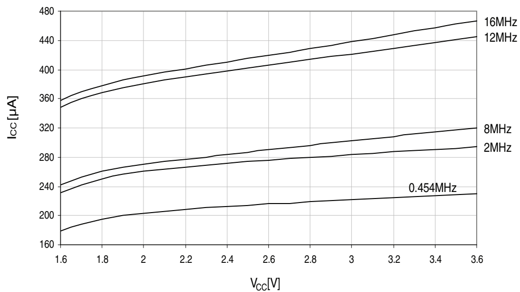
Figure 37-275. Standby supply current vs. V_{CC} .
