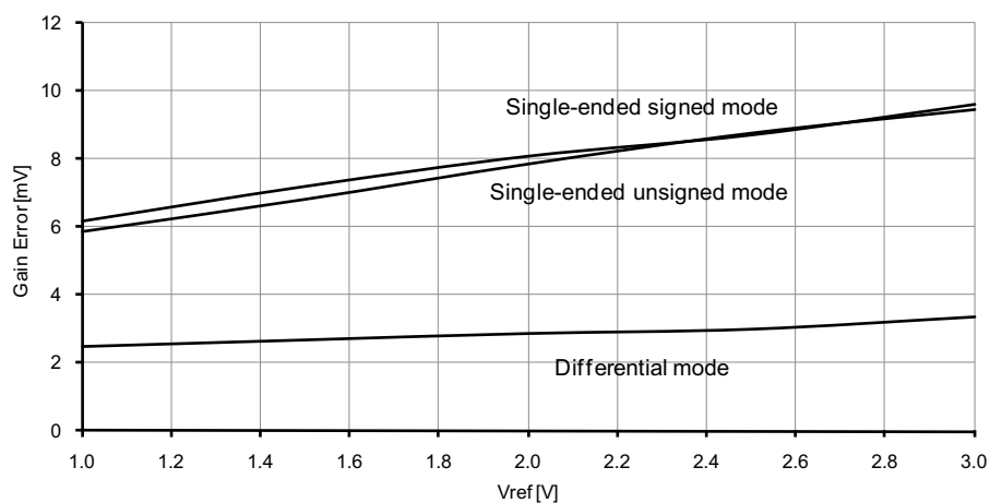
Figure 37-212. Gain error vs. V_{REF} . T = 25^\circ\text{C} , V_{CC} = 3.6\text{V} , ADC sampling speed = 500ksps.
