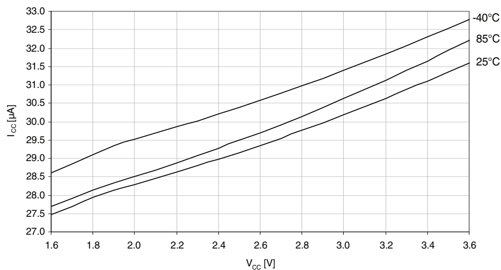
Figure 37-95. Idle mode supply current vs. V_{\text{CC}} .
