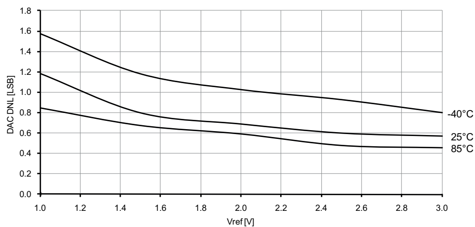
Figure 37-220. DNL error vs. V_{REF} . V_{CC} = 3.6V .
