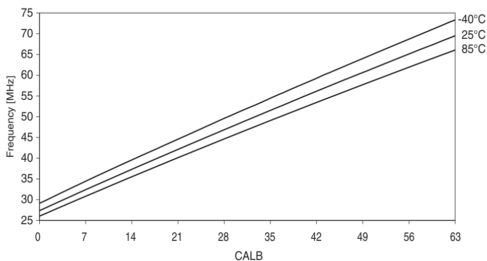
Figure 37-79. 32MHz internal oscillator frequency vs. CALB calibration value.
