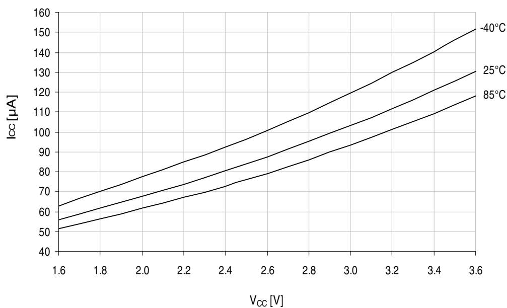
Figure 37-4. Active mode supply current vs. V_{CC} .
