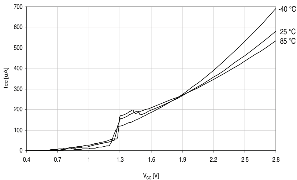
Figure 37-68. Power-on reset current consumption vs. V_{CC} .
