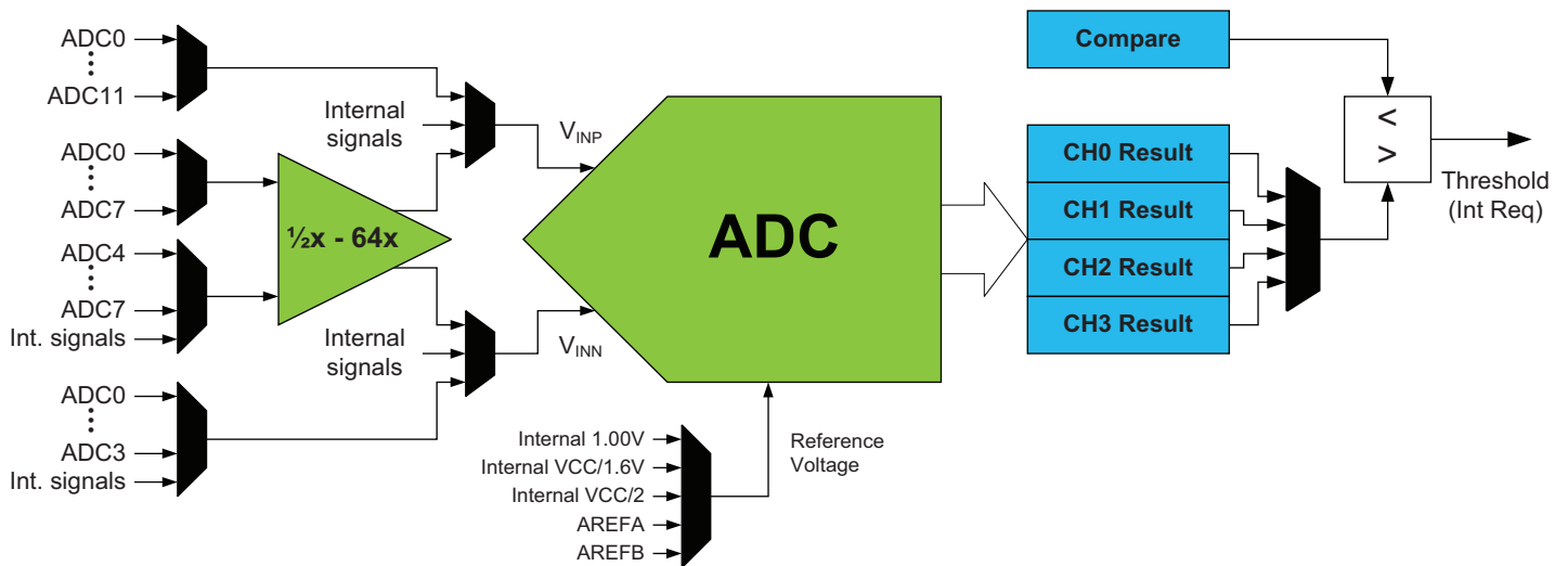
Figure 28-1. ADC overview.
