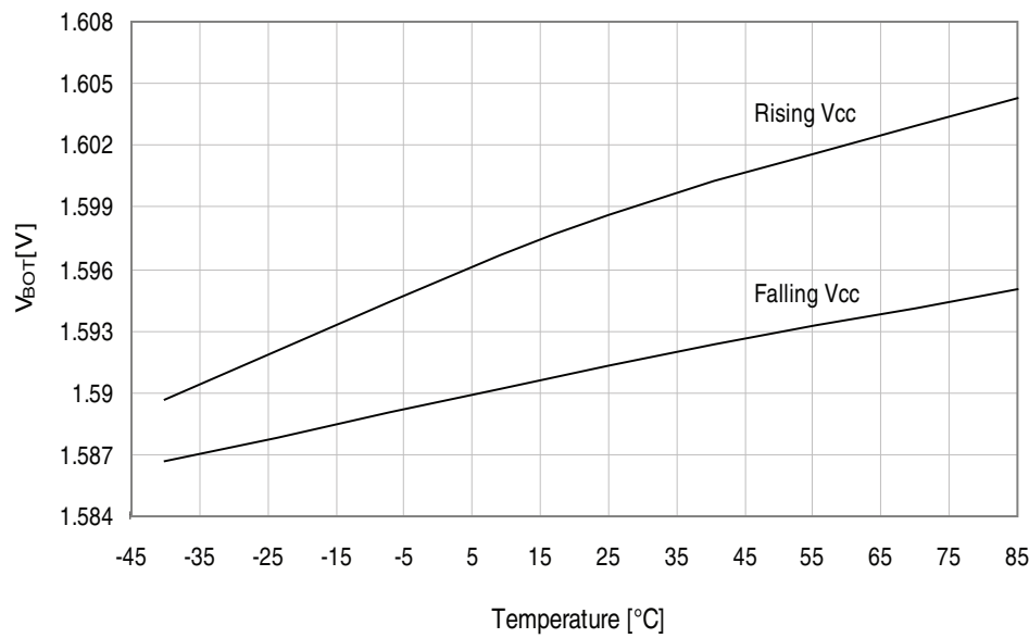
Figure 37-315. BOD thresholds vs. temperature. BOD level = 1.6V.
