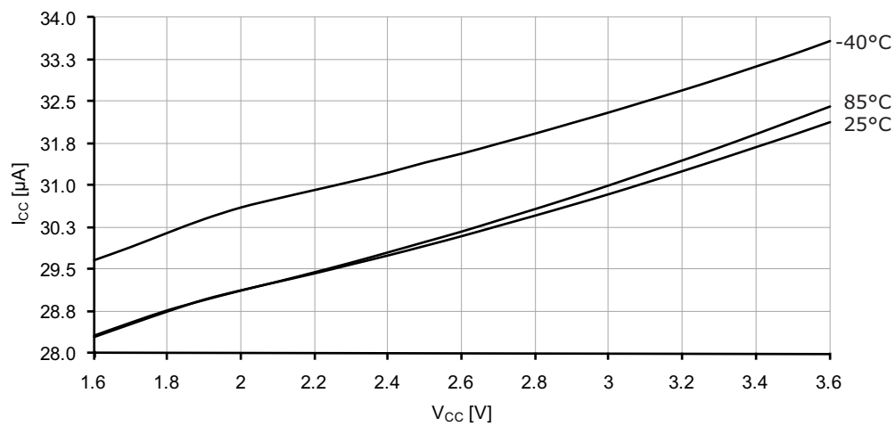
Figure 37-180. Idle mode supply current vs. V_{\text{CC}} .
