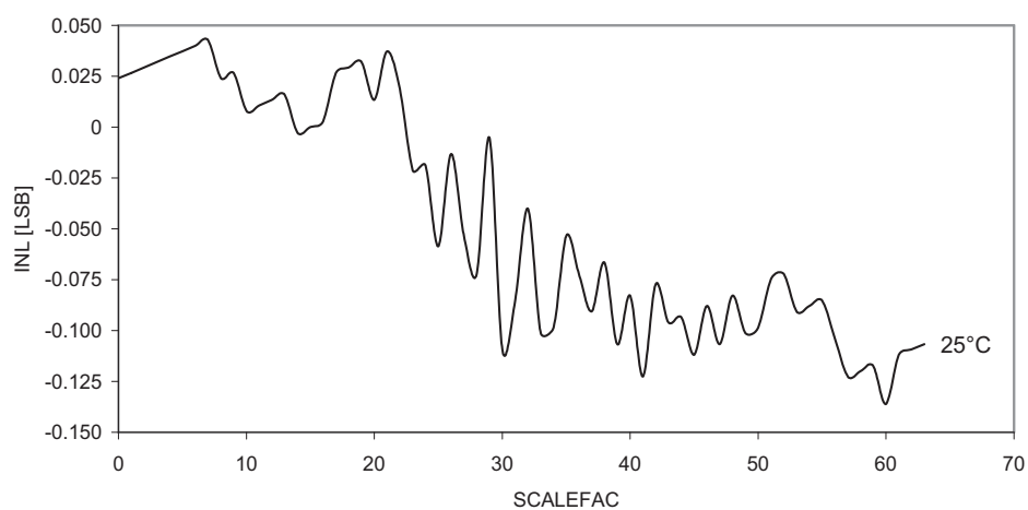
Figure 37-143. Voltage scaler INL vs. SCALEFAC.
