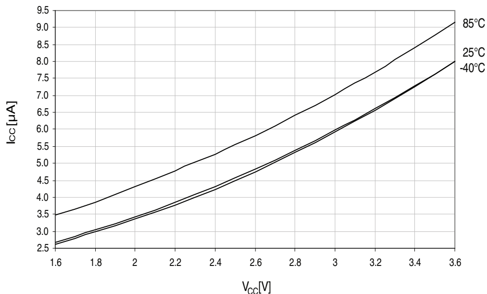
Figure 37-20. Standby supply current vs. V_{CC} .
