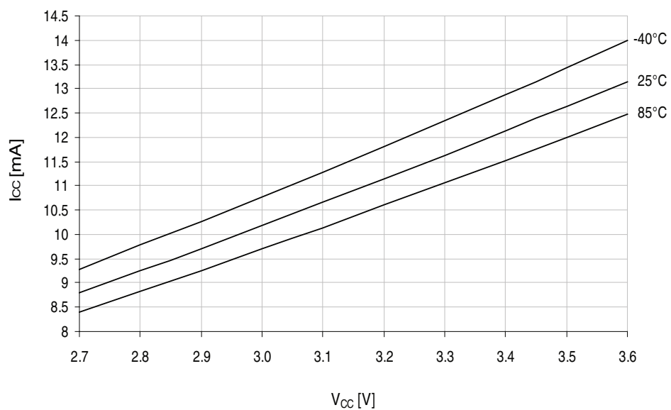
Figure 37-7. Active mode supply current vs. V_{CC} . f_{SYS} = 32\text{MHz} internal oscillator.
