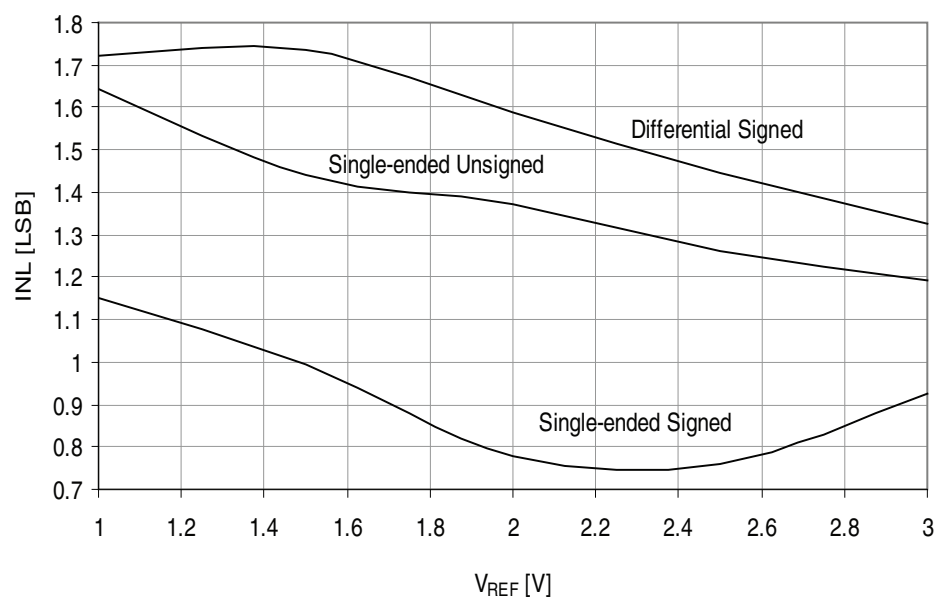
Figure 37-36. INL error vs. external V_{REF} .
