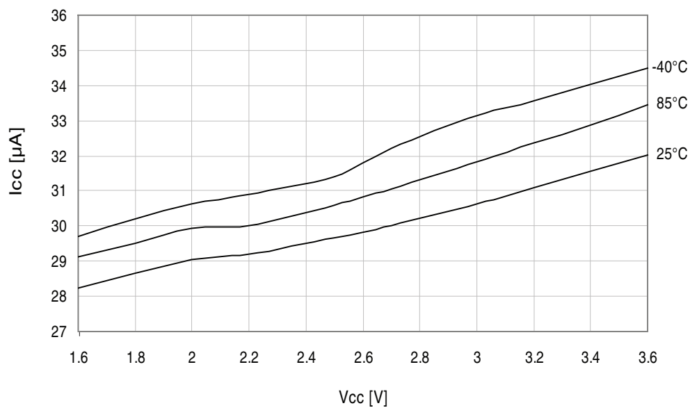
Figure 37-265. Idle mode supply current vs. V_{\text{CC}} .
