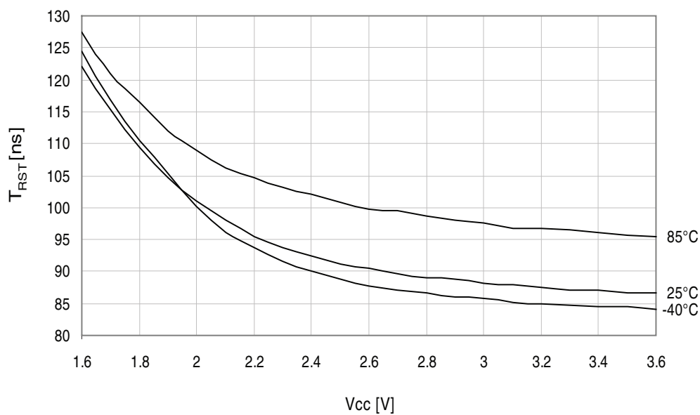
Figure 37-317. Minimum Reset pin pulse width vs. V_{CC} .
