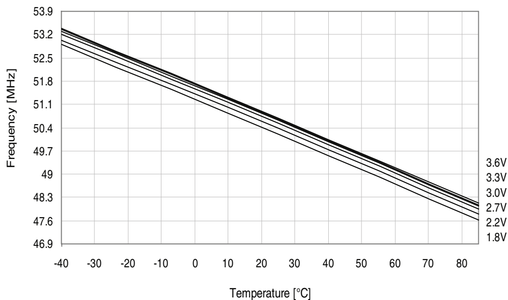
Figure 37-335. 48MHz internal oscillator frequency vs. temperature.
