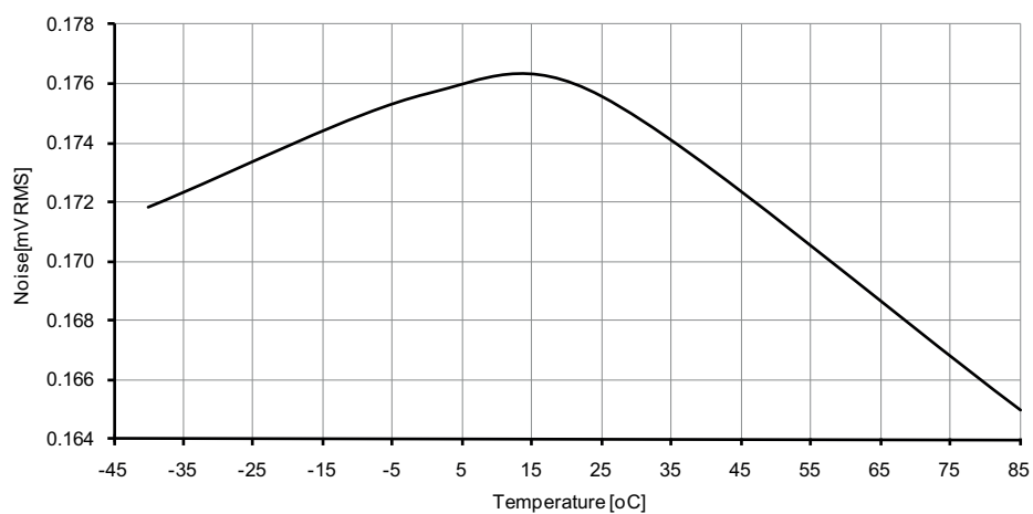
Figure 37-221. DAC noise vs. temperature.
