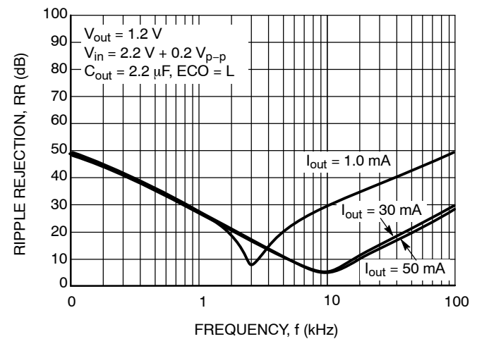
Figure 27. Ripple Rejection vs. Frequency
