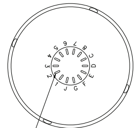
14X SOLDER TERMINALS SOLDER WIRE USING SN63. MAXIMUM TEMP 210°C FOR NO MORE THAN 5 SEC.
