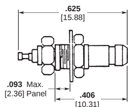
8-32 UNC-2A (Modified) Receptacle, Rear Mount Part Number 145-0003-0001
