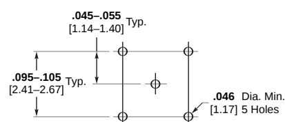
Small Pattern Connectors 141-0019-0001 and 141-0023-0001 Only
