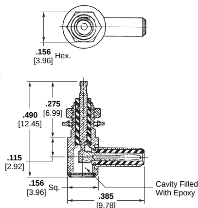
Right-Angle Receptacle Mounting Hole Shown Below Part Number 141-1012-0001
