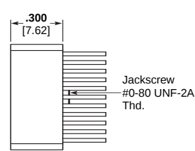
Plug
