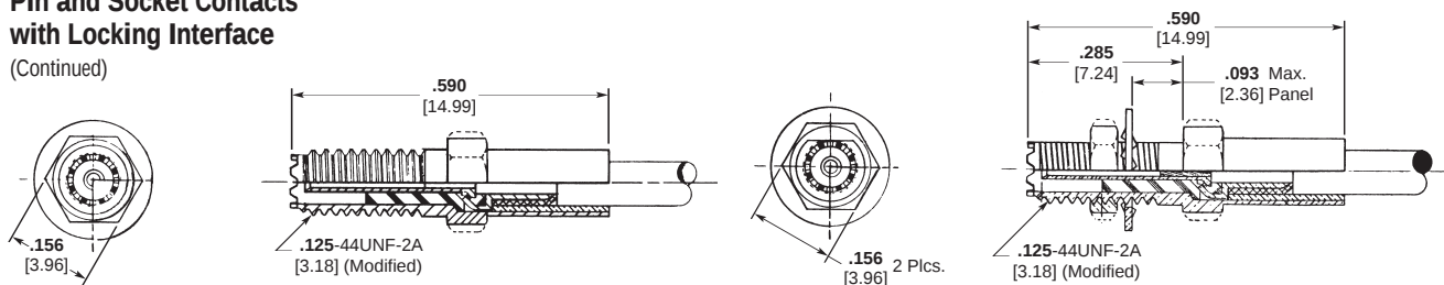
Straight Jack 1 Part Number 141-0017-0001 Instruction Sheet Number 408-08510 Former MICRODOT I.S. Number RF-ASMB-12
