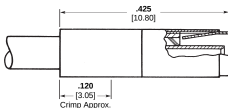
Part Number 142-1500-0001 CS Socket
