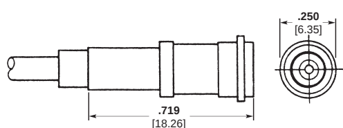
Straight Plug Part Number 144-0001-0001
