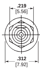
Receptacle, Front Mount Part Number 145-0002-0001
