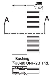
Section A-A Plug
