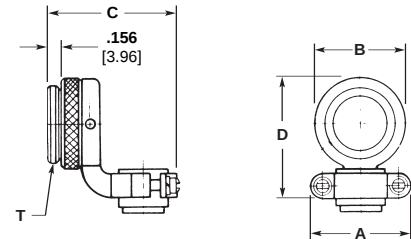
Right-Angle
