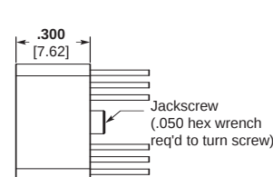
Plug
