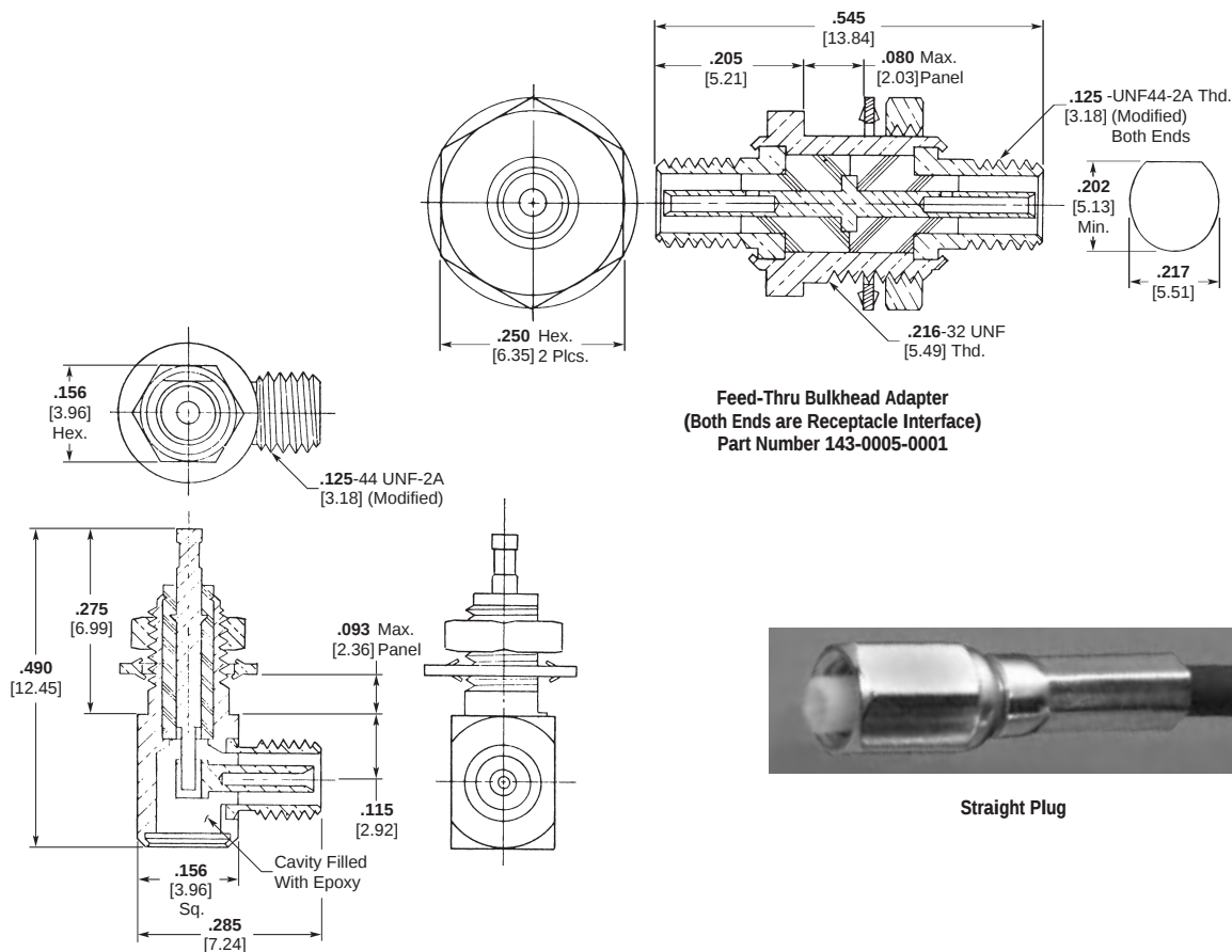
Right-Angle Receptacle 1 Part Number 141-0013-0001
