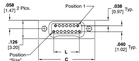
Receptacle with Flying Leads Drawing Number 1589476
