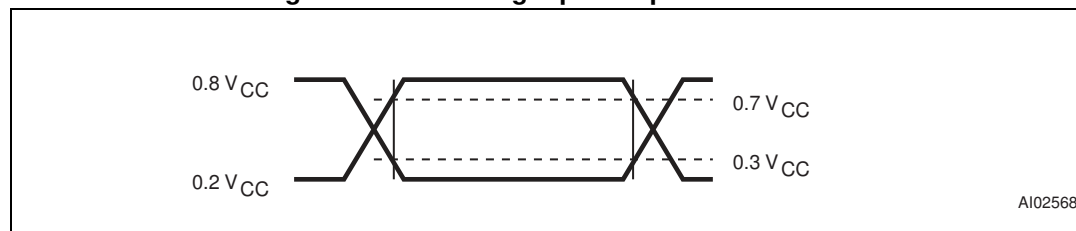
Figure 35. AC testing input/output waveforms
