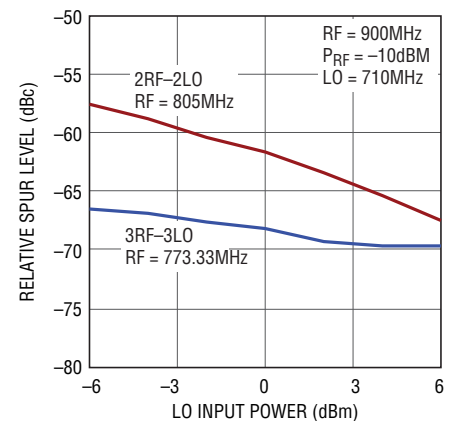
2 \times 2 and 3 \times 3 Spur Suppression vs LO Power
