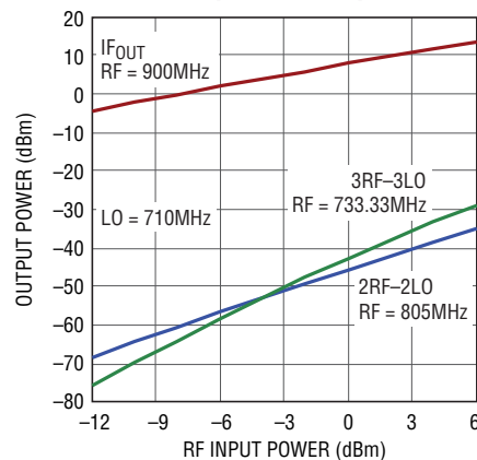
Single-Tone IF Output Power, 2 \times 2 and 3 \times 3 Spurs vs RF Input Power
