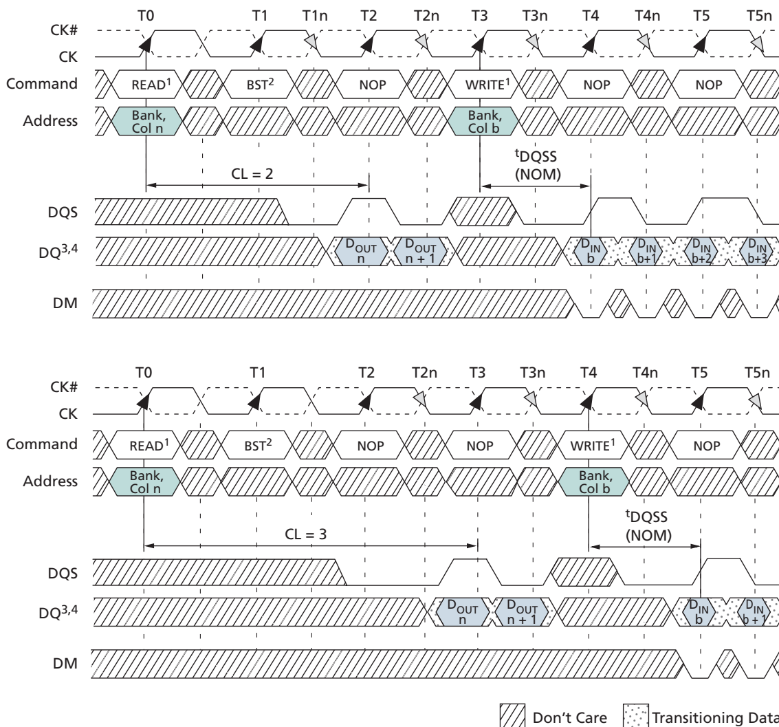
Figure 29: READ-to-WRITE
