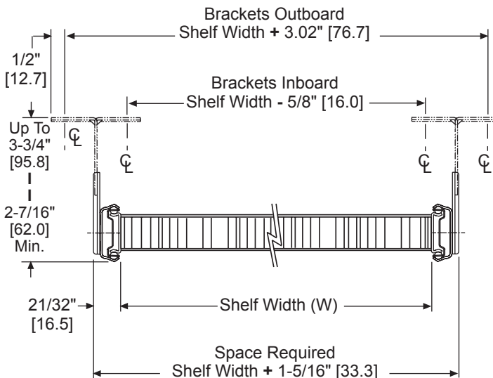
Mounting Hole Centerlines, Front Elevation
