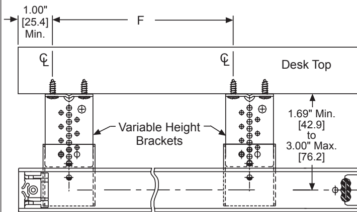
Mounting Hole Centerlines, Side Elevation
