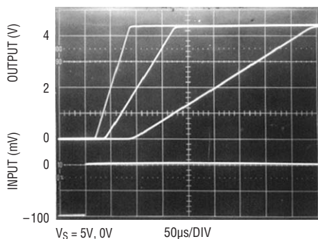
V S = 5V, 0V 50ns/DIV
