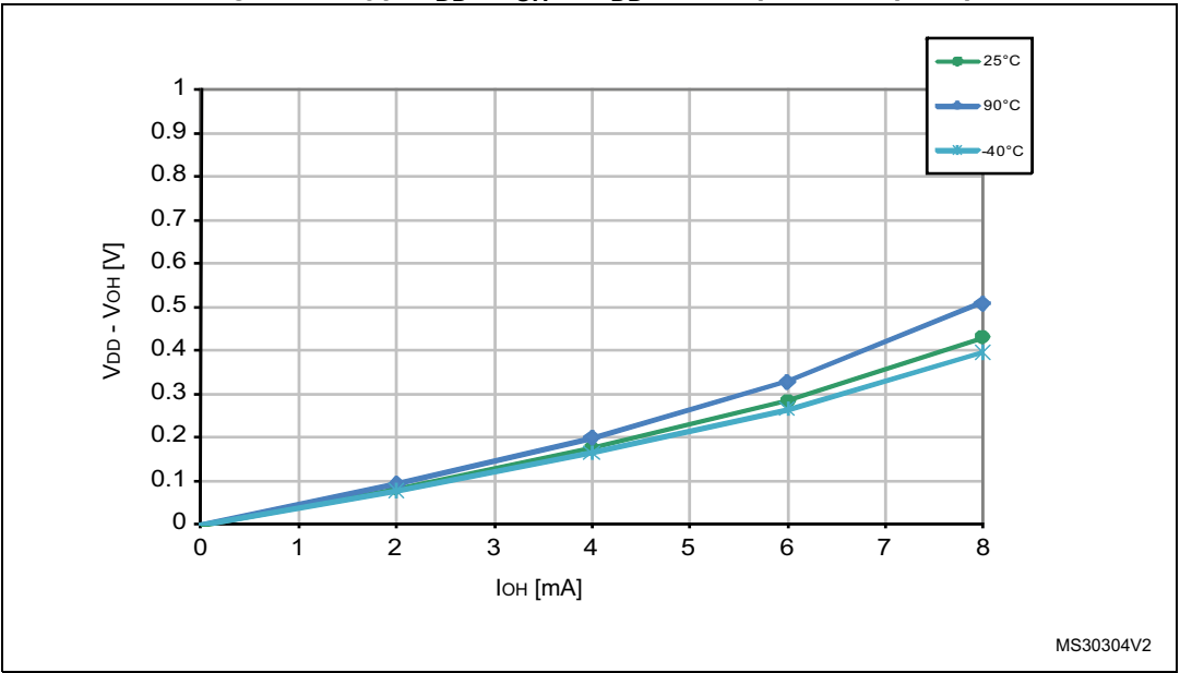
Figure 21. Typ. V_{DD} - V_{OH} at V_{DD} = 1.8 V (standard ports)
