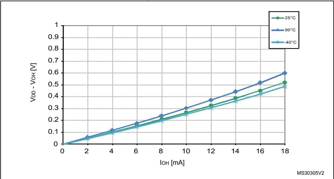
Figure 22. Typ. V_{DD} - V_{OH} at V_{DD} = 3.0\text{ V} (standard ports)
