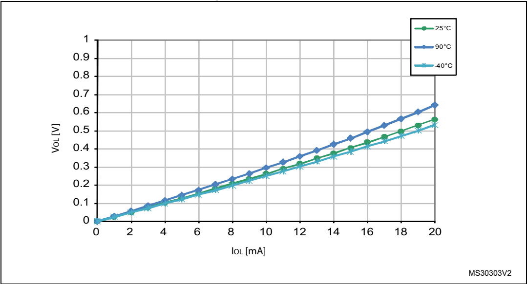
Figure 20. Typ. V_{OL} at V_{DD} = 3.0 V (standard ports)
