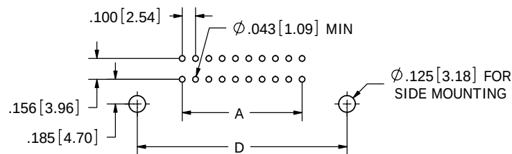
PCB LAYOUT
