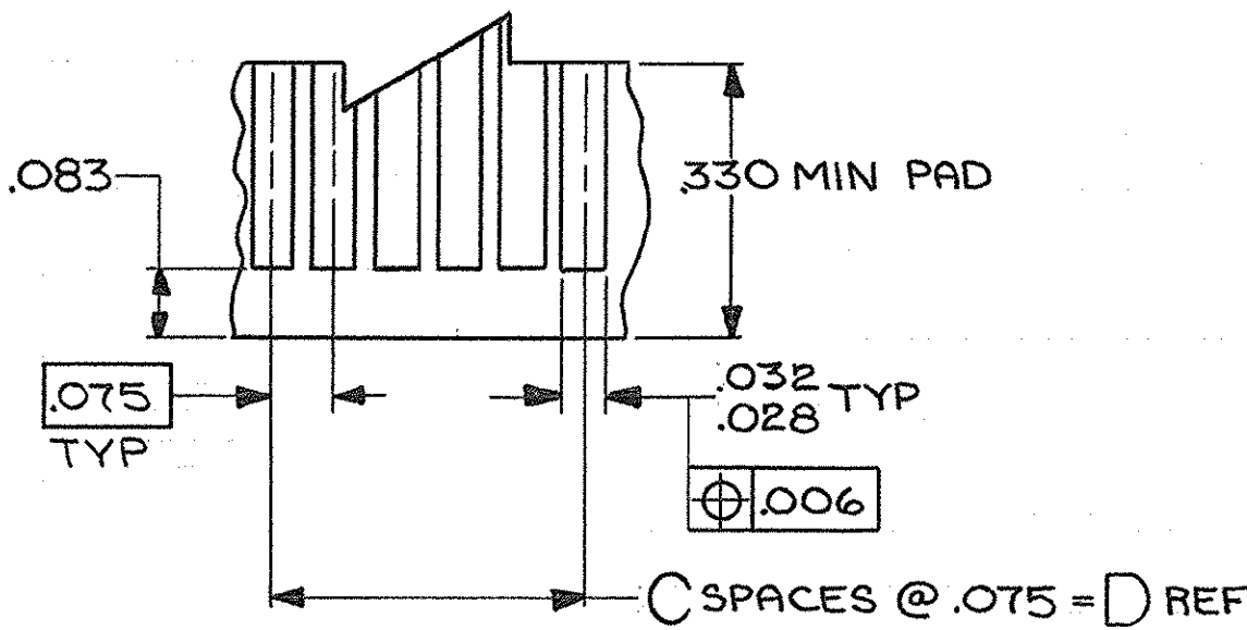
RECOMMENDED PRINTED CIRCUIT BOARD LAYOUT
