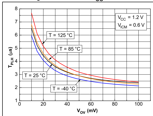
Figure 25. Propagation delay T_{PLH} vs. input signal overdrive at V_{CC} = 1.2\text{ V}
