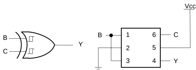
Configuration 5 2-Input XOR Gate
