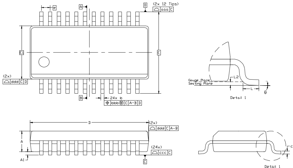
Figure 16. 24-Pin SSOP
