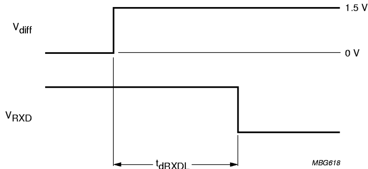
Fig.7 Timing diagram for bus dominant to RXD low.
