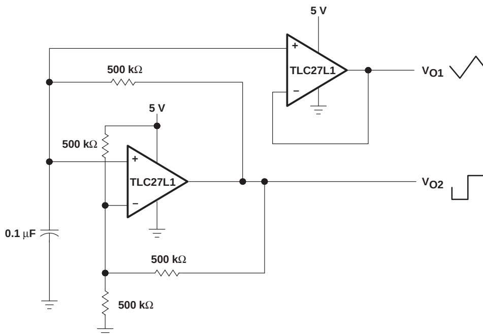
Figure 49. Multivibrator
