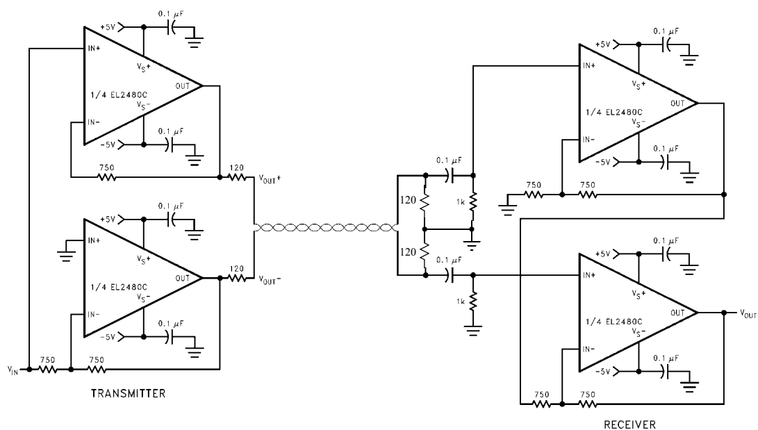
DIFFERENTIAL LINE-DRIVER/RECEIVER
