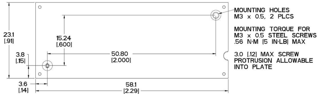
Top View
