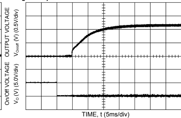
Figure 41. Typical Start-up Using Remote On/Off, negative logic version shown ( V_{IN} = V_{IN,NOM} , I_o = I_{o,max} ).
