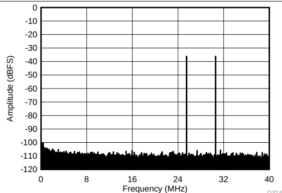
Figure 76. FFT FOR Two-Tone Input Signal ( -36\text{ dBFS} at 185 MHz and 190 MHz)
