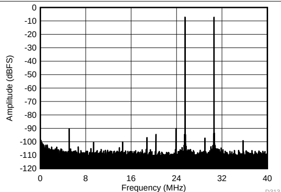
Figure 75. FFT FOR Two-Tone Input Signal ( -7\text{ dBFS} at 185 MHz and 190 MHz)
