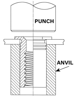
REQUIRED INSTALLATION ANVIL FOR SHEETS BELOW .032" / 0.81 mm
