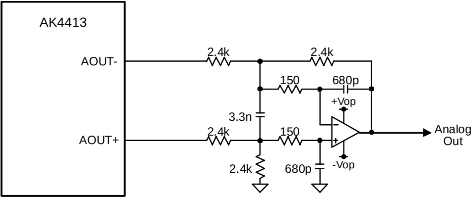
Figure 21. External LPF Circuit Example 1 for PCM (fc = 125kHz, Q=0.692)
