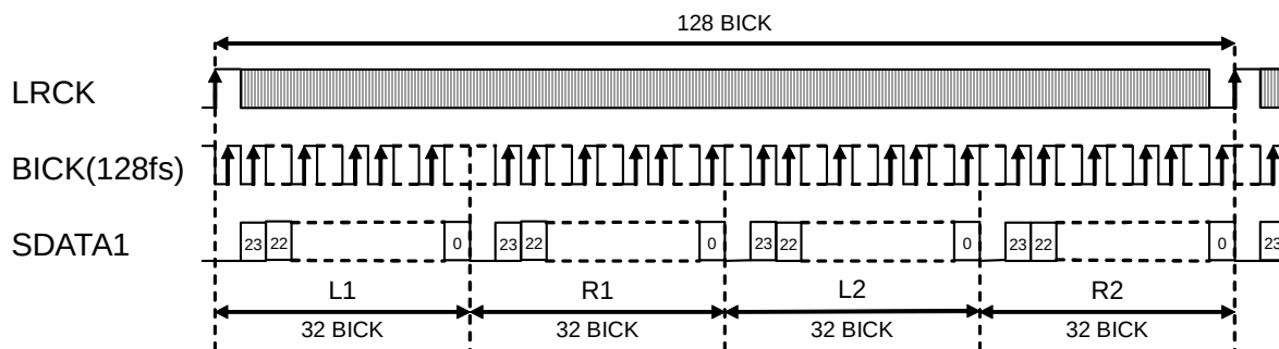
Figure 10. Mode 16 Timing
